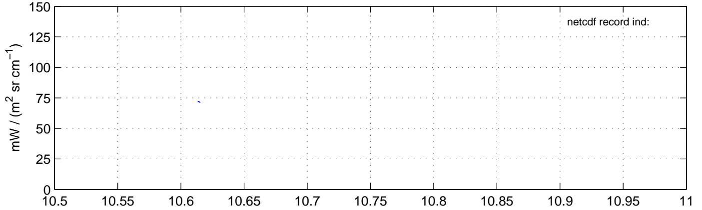
sh130920 Mean Radiance 1093.00 – 1097.00, good segments
