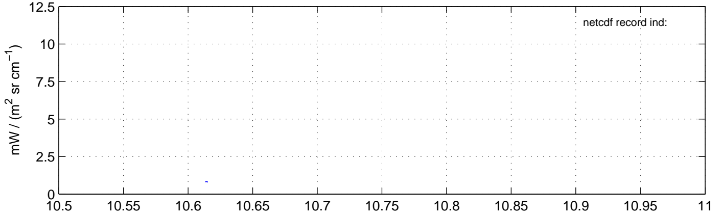
sh130920 Mean Radiance 2500.00 – 2510.00, good segments
