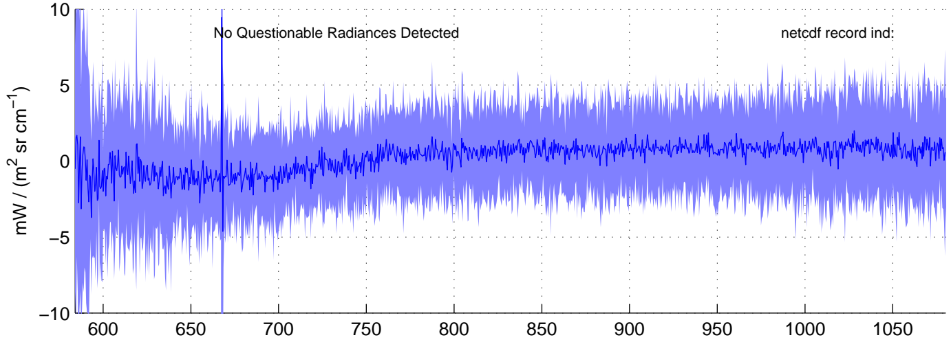
sh130920, Questionable (IMAG) LW Radiances included in shis_130920_sci_lw.nc BLUE = OK (meaned by seg); RED = significant imaginary content
