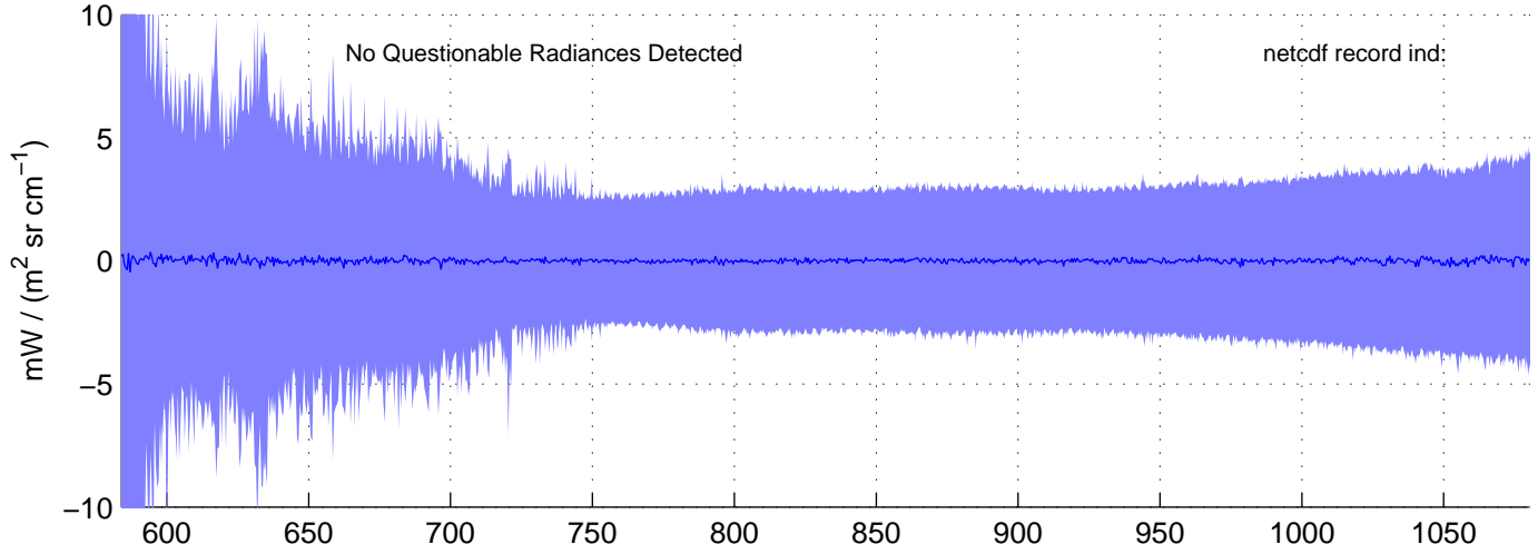
sh130919, Questionable (IMAG) LW Radiances included in shis_130919_sci_lw.nc BLUE = OK (meaned by seg); RED = significant imaginary content
