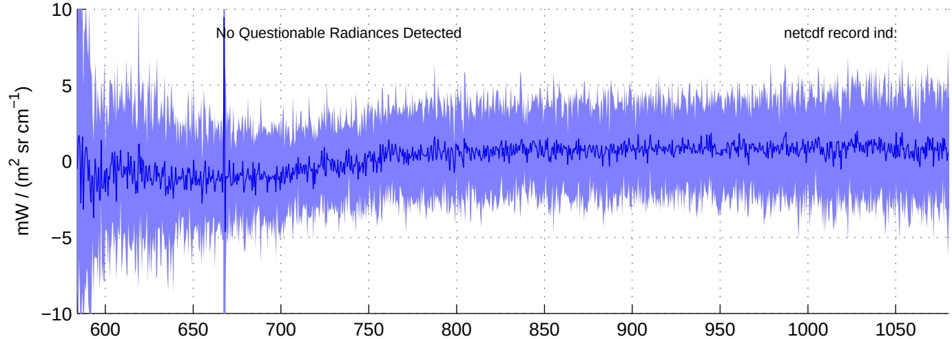
sh130920, Questionable (IMAG) LW Radiances included in shis_130920_sci_lw.nc BLUE = OK (meaned by seg); RED = significant imaginary content
