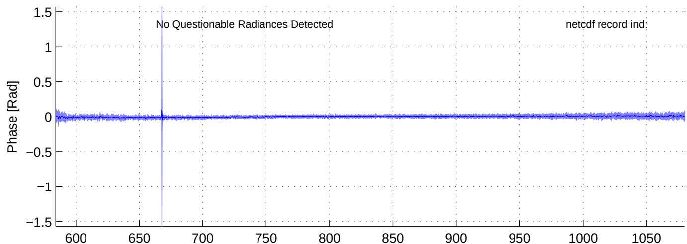
sh130920, PHASE(LW) Radiances included in shis_130920_sci_lw.nc BLUE = OK (meaned by seg); RED = significant imaginary content
