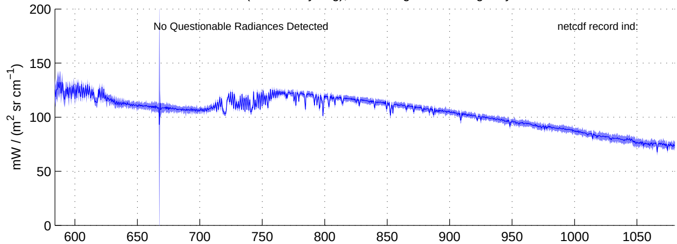
sh130920, REAL(LW) Radiances included in shis_130920_sci_lw.nc BLUE = OK (meaned by seg); RED = significant imaginary content
