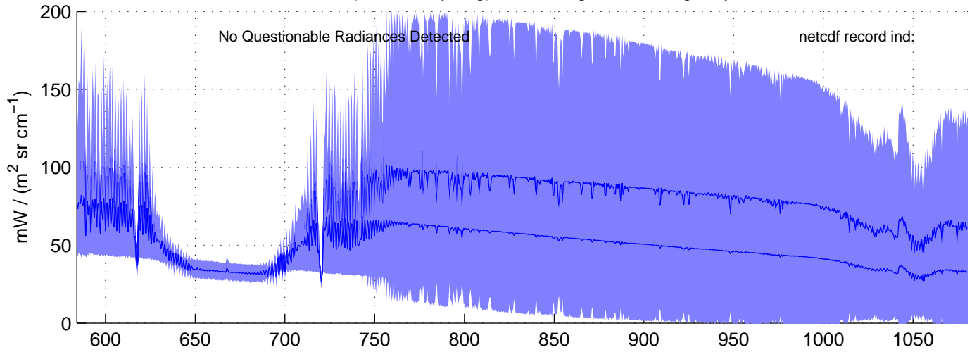
sh130916, REAL(LW) Radiances included in shis_130916_sci_lw.nc BLUE = OK (meaned by seg); RED = significant imaginary content
