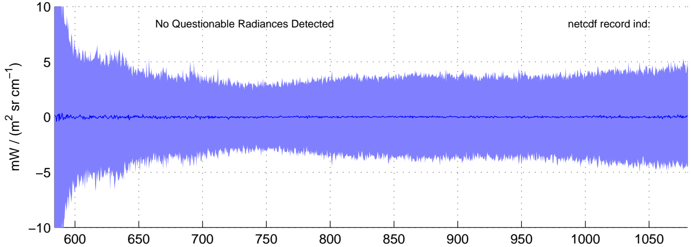
sh130916, Questionable (IMAG) LW Radiances included in shis_130916_sci_lw.nc BLUE = OK (meaned by seg); RED = significant imaginary content
