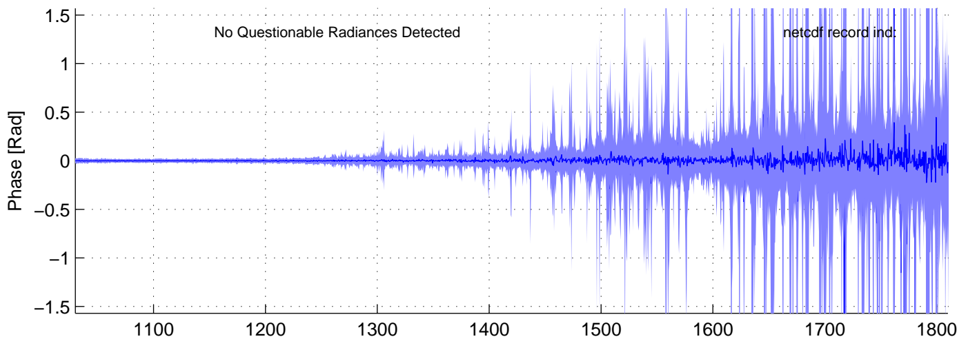
sh130917, PHASE(MW) Radiances included in shis_130917_sci_mw.nc BLUE = OK (meaned by seg); RED = significant imaginary content
