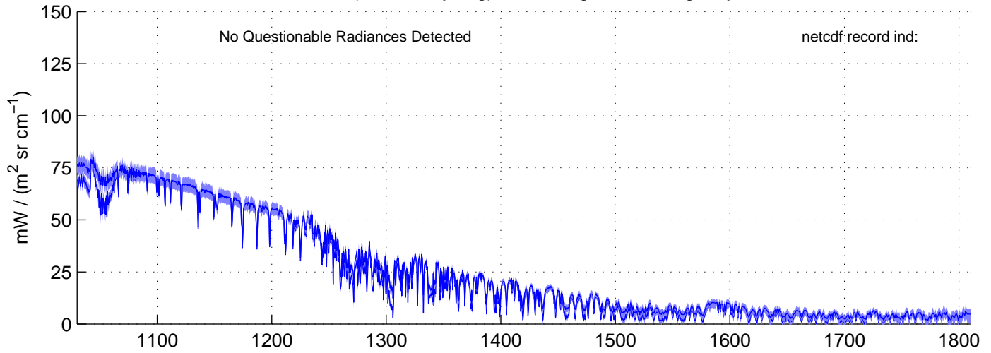
sh130917, REAL(MW) Radiances included in shis_130917_sci_mw.nc BLUE = OK (meaned by seg); RED = significant imaginary content
