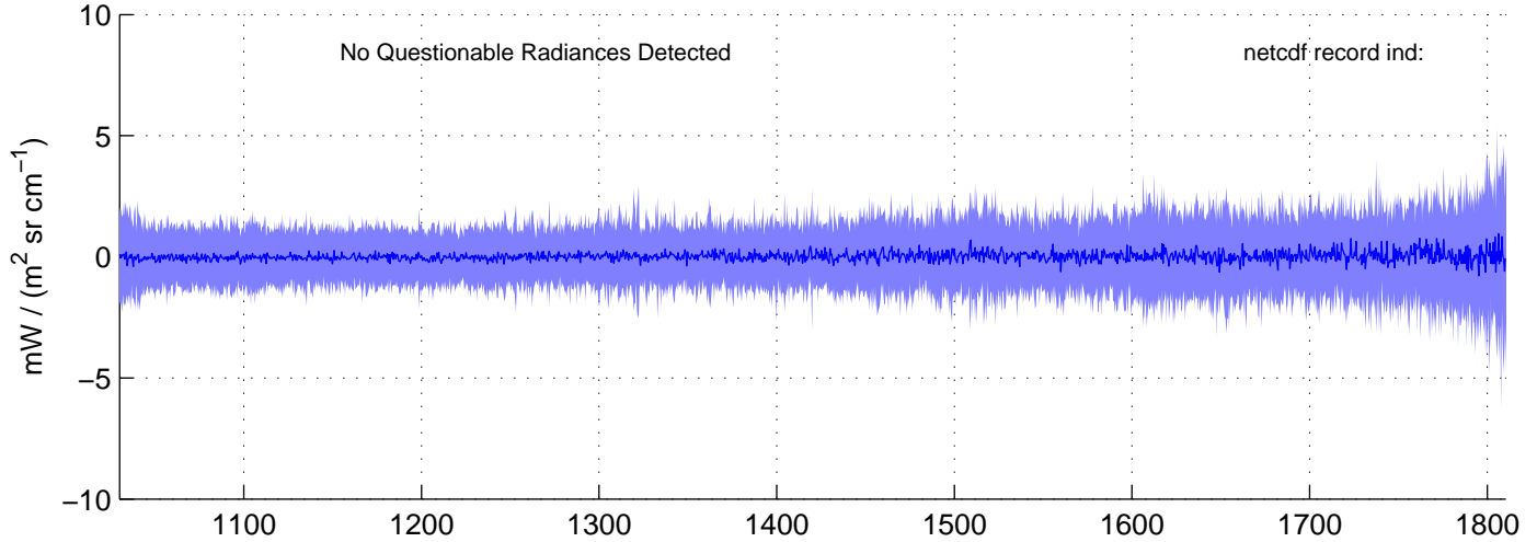
sh130917, IMAG(MW) Radiances included in shis_130917_sci_mw.nc BLUE = OK (meaned by seg); RED = significant imaginary content
