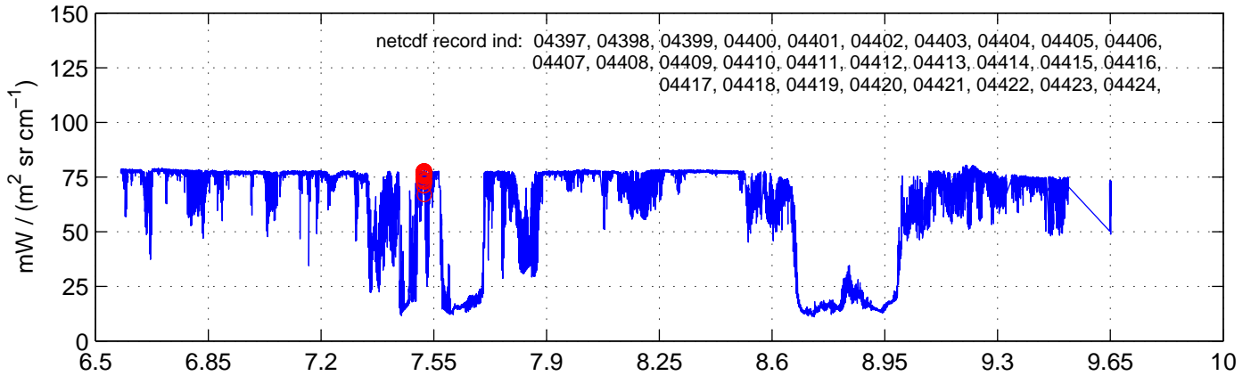
sh130917 Mean Radiance 1093.00 – 1097.00, good segments
