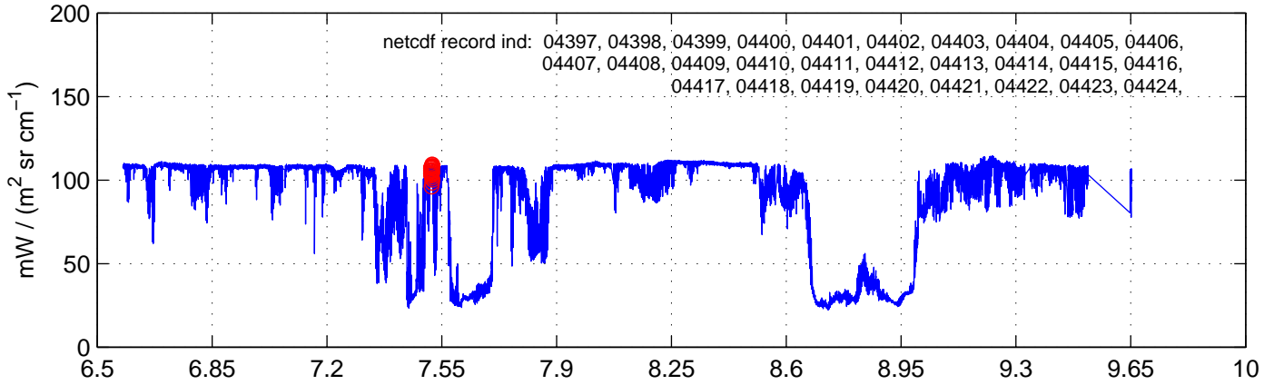
sh130917 Mean Radiance 895.00 – 900.00, good segments
