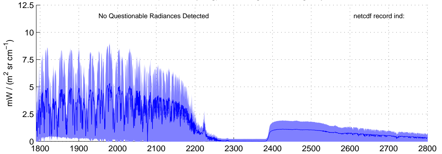
sh130917, REAL(SW) Radiances included in shis_130917_sci_sw.nc BLUE = OK (meaned by seg); RED = significant imaginary content
