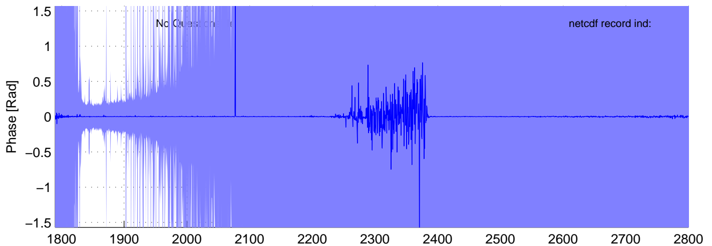
sh130917, PHASE(SW) Radiances included in shis_130917_sci_sw.nc BLUE = OK (meaned by seg); RED = significant imaginary content
