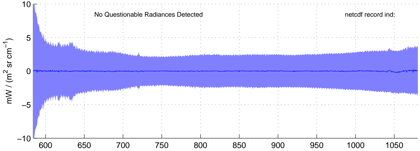
sh130917, Questionable (IMAG) LW Radiances included in shis_130917_sci_lw.nc BLUE = OK (meaned by seg); RED = significant imaginary content
