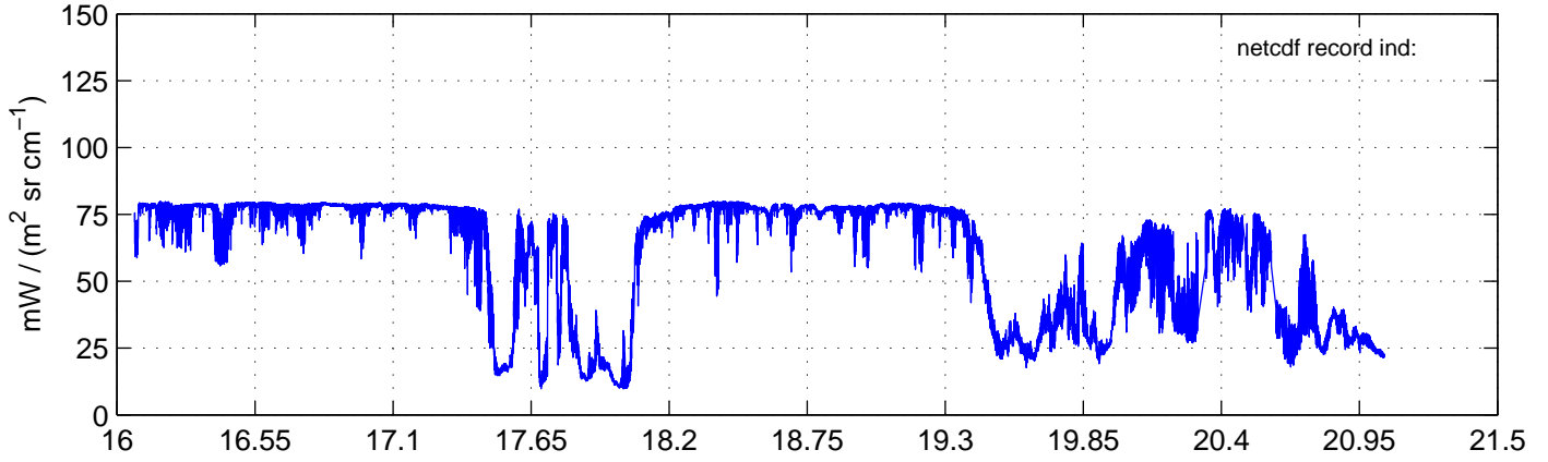
sh130916 Mean Radiance 1093.00 – 1097.00, good segments
