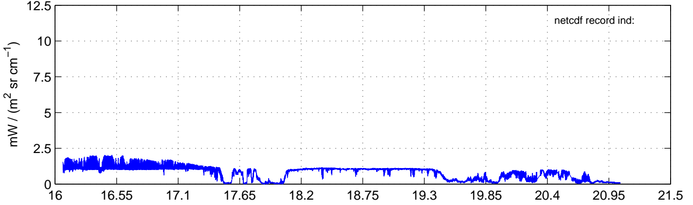
sh130916 Mean Radiance 2500.00 – 2510.00, good segments
