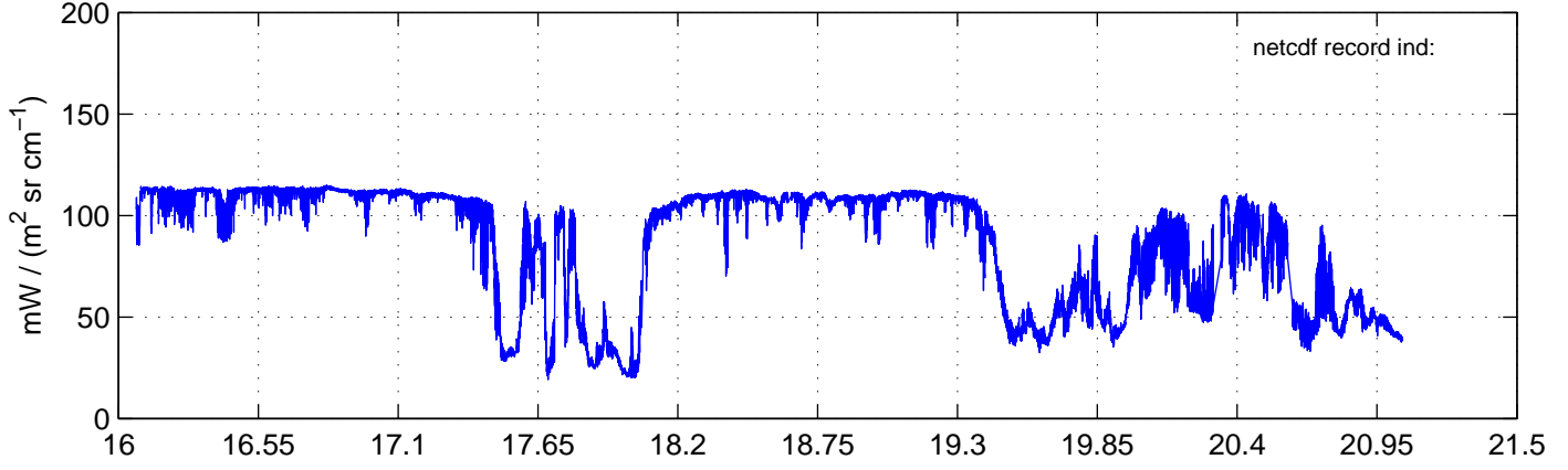
sh130916 Mean Radiance 895.00 – 900.00, good segments
