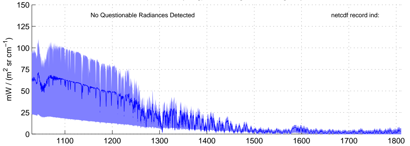
sh130916, REAL(MW) Radiances included in shis_130916_sci_mw.nc BLUE = OK (meaned by seg); RED = significant imaginary content
