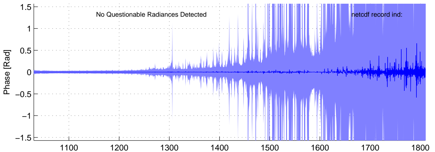
sh130916, PHASE(MW) Radiances included in shis_130916_sci_mw.nc BLUE = OK (meaned by seg); RED = significant imaginary content
