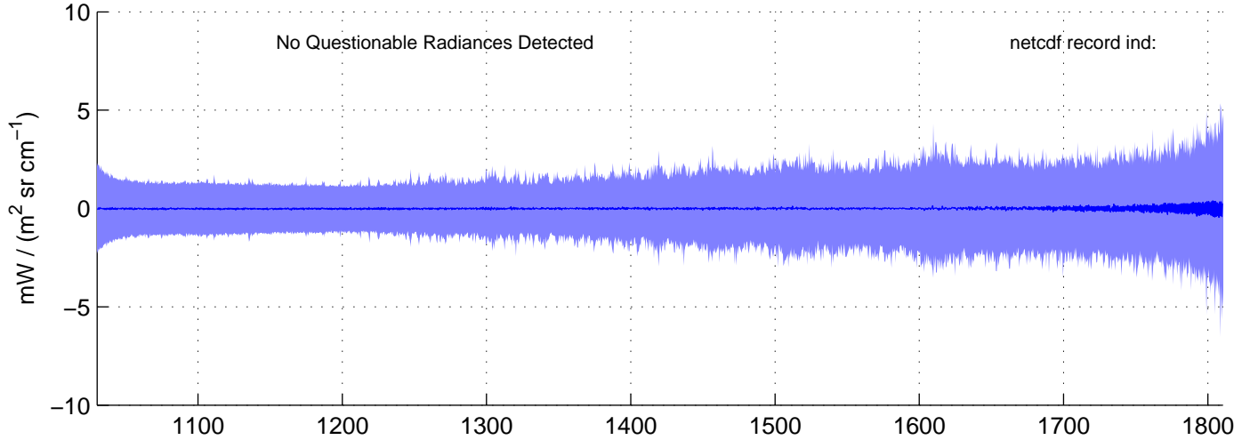
sh130916, IMAG(MW) Radiances included in shis_130916_sci_mw.nc BLUE = OK (meaned by seg); RED = significant imaginary content
