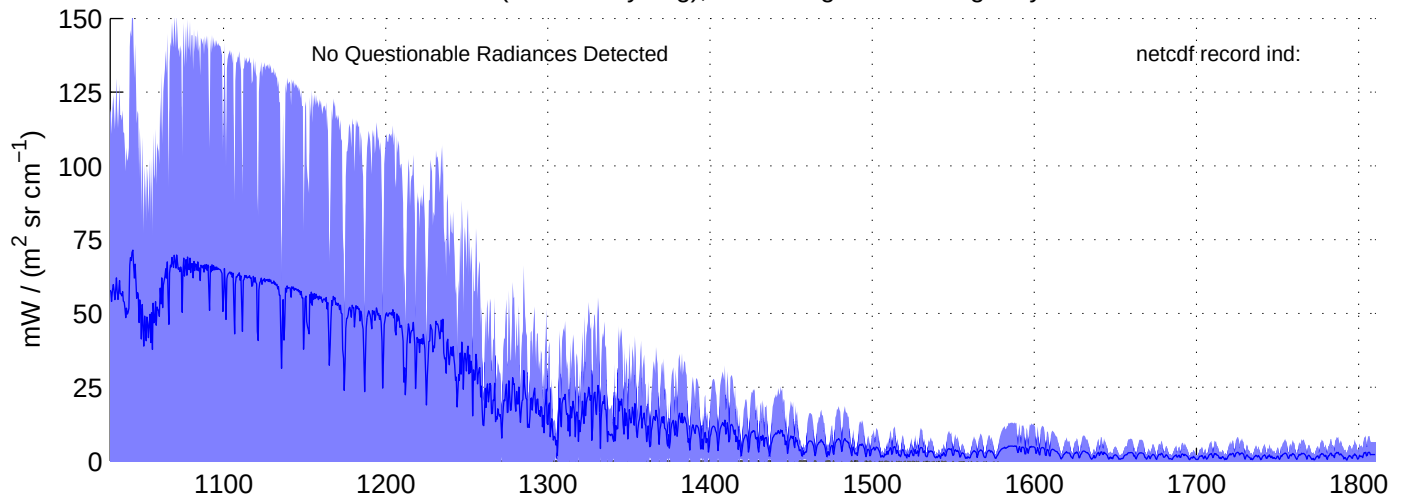
sh130905, REAL(MW) Radiances included in shis_130905_sci_mw.nc BLUE = OK (meaned by seg); RED = significant imaginary content
