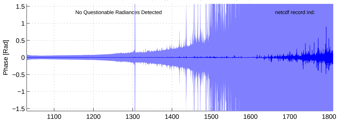
sh130905, PHASE(MW) Radiances included in shis_130905_sci_mw.nc BLUE = OK (meaned by seg); RED = significant imaginary content
