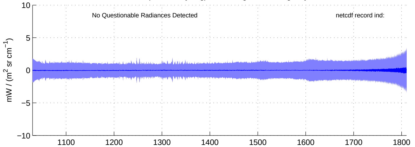
sh130905, IMAG(MW) Radiances included in shis_130905_sci_mw.nc BLUE = OK (meaned by seg); RED = significant imaginary content
