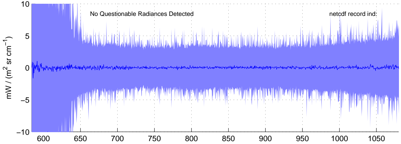
sh130905, Questionable (IMAG) LW Radiances included in shis_130905_sci_lw.nc BLUE = OK (meaned by seg); RED = significant imaginary content
