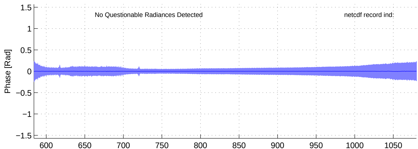
sh130905, PHASE(LW) Radiances included in shis_130905_sci_lw.nc BLUE = OK (meaned by seg); RED = significant imaginary content
