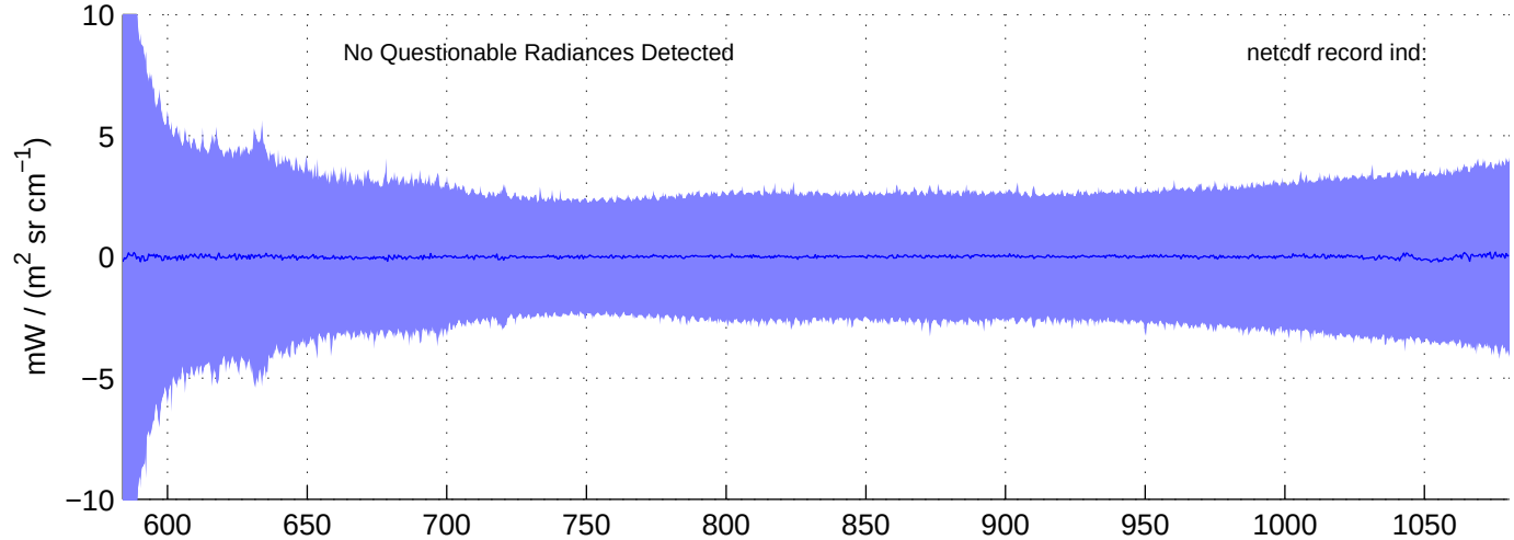
sh130905, Questionable (IMAG) LW Radiances included in shis_130905_sci_lw.nc BLUE = OK (meaned by seg); RED = significant imaginary content
