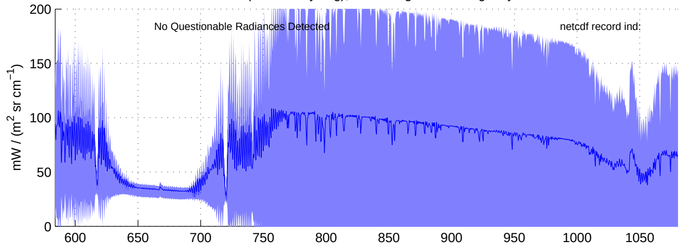
sh130905, REAL(LW) Radiances included in shis_130905_sci_lw.nc BLUE = OK (meaned by seg); RED = significant imaginary content
