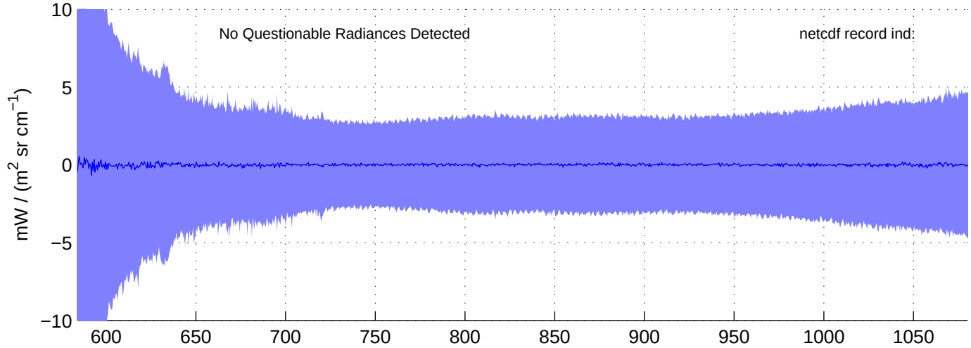
sh130904, Questionable (IMAG) LW Radiances included in shis_130904_sci_lw.nc BLUE = OK (meaned by seg); RED = significant imaginary content
