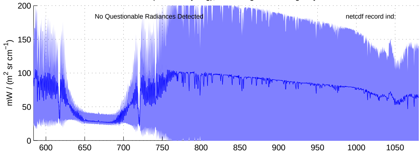
sh130904, REAL(LW) Radiances included in shis_130904_sci_lw.nc BLUE = OK (meaned by seg); RED = significant imaginary content
