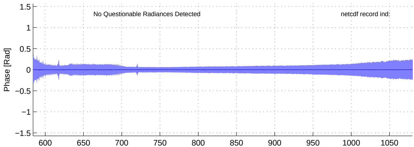
sh130904, PHASE(LW) Radiances included in shis_130904_sci_lw.nc BLUE = OK (meaned by seg); RED = significant imaginary content
