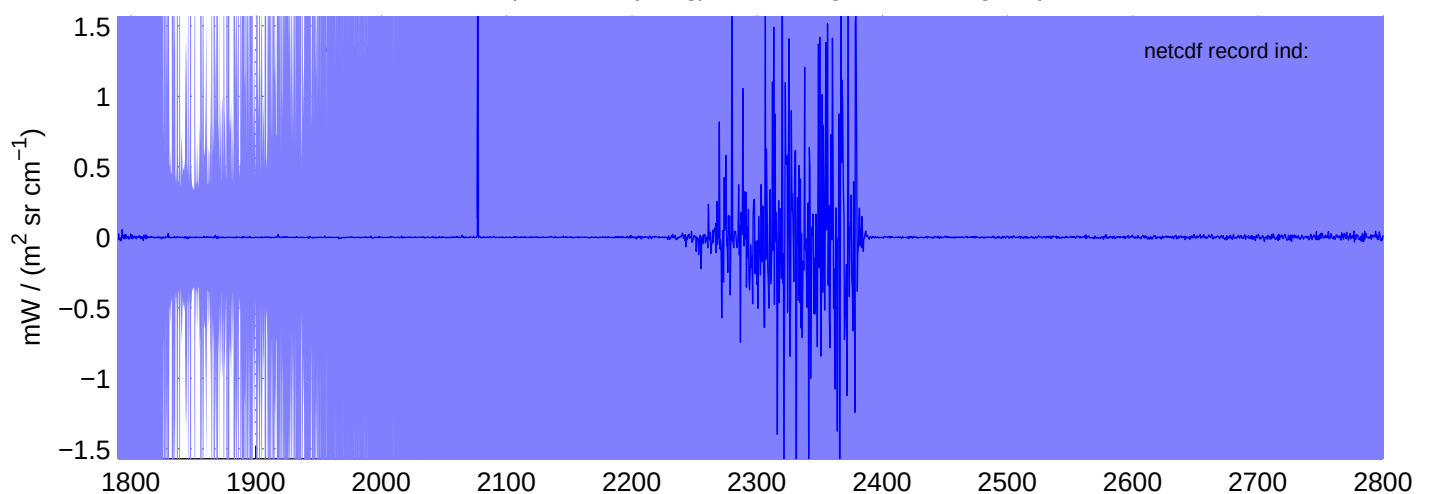
sh130904, PHASE(SW) Radiances included in shis_130904_sci_sw.nc BLUE = OK (meaned by seg); RED = significant imaginary content
