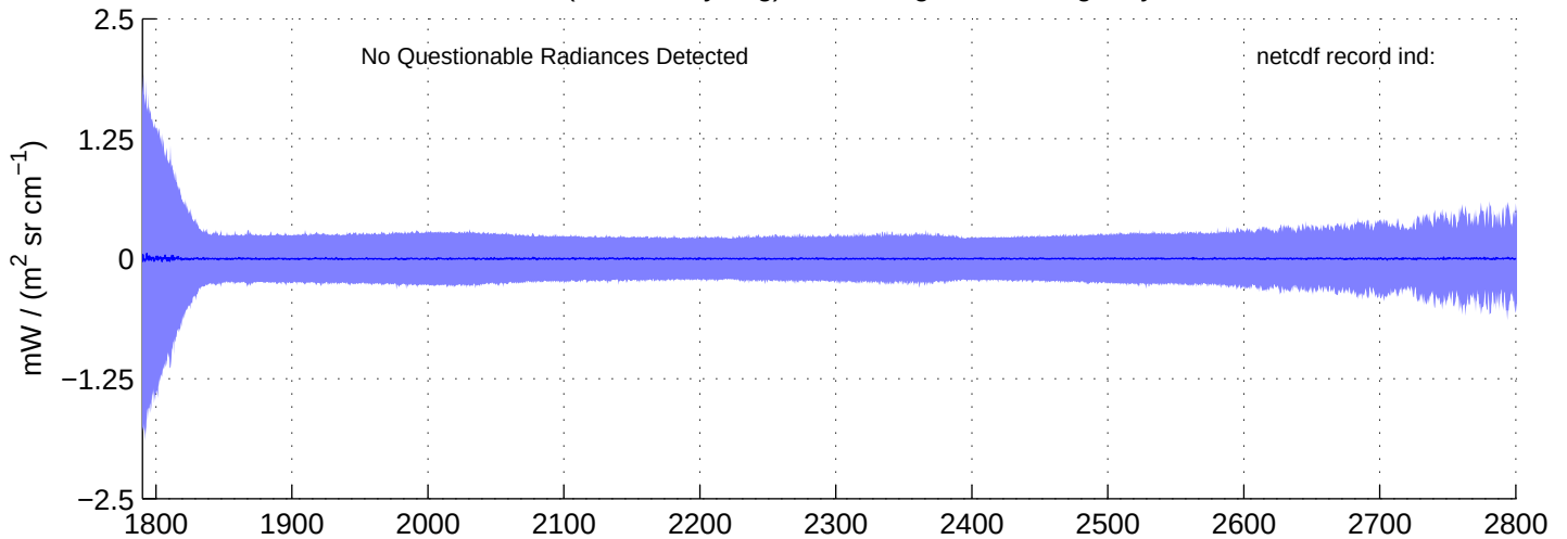
sh130904, IMAG(SW) Radiances included in shis_130904_sci_sw.nc BLUE = OK (meaned by seg); RED = significant imaginary content
