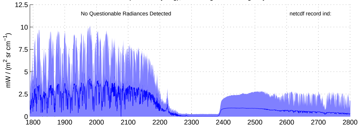
sh130904, REAL(SW) Radiances included in shis_130904_sci_sw.nc BLUE = OK (meaned by seg); RED = significant imaginary content
