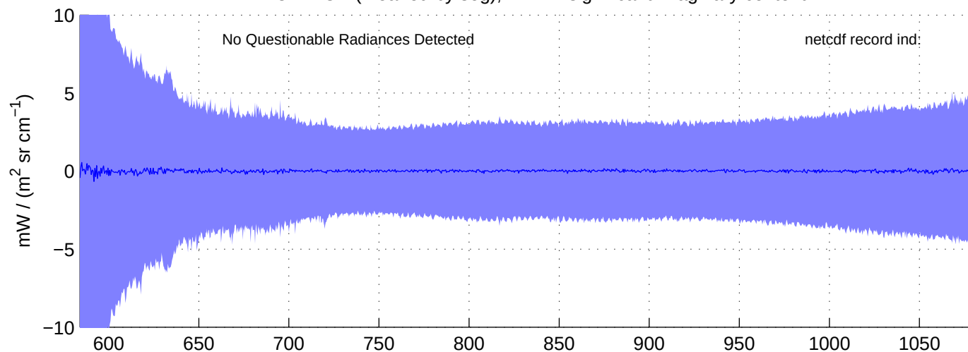
sh130904, Questionable (IMAG) LW Radiances included in shis_130904_sci_lw.nc BLUE = OK (meaned by seg); RED = significant imaginary content
