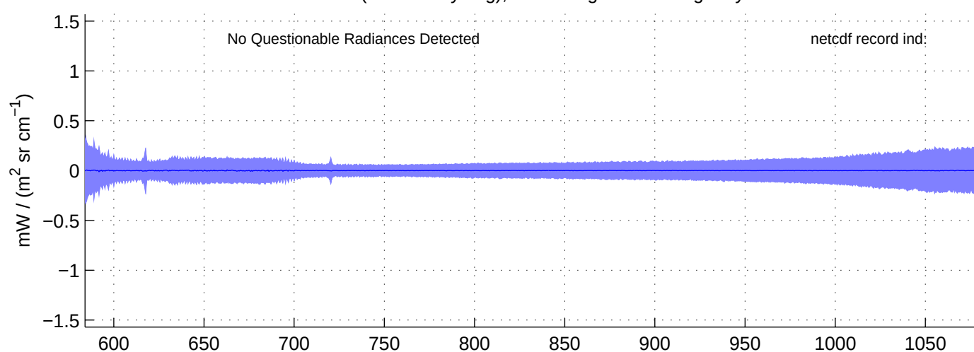
sh130904, PHASE(LW) Radiances included in shis_130904_sci_lw.nc BLUE = OK (meaned by seg); RED = significant imaginary content
