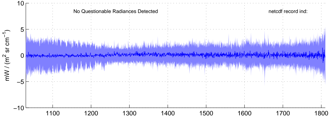
sh130830, IMAG(MW) Radiances included in shis_130830_sci_mw.nc BLUE = OK (meaned by seg); RED = significant imaginary content
