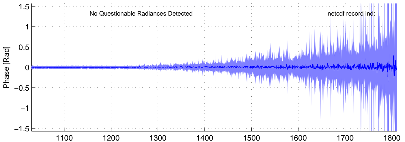
sh130830, PHASE(MW) Radiances included in shis_130830_sci_mw.nc BLUE = OK (meaned by seg); RED = significant imaginary content
