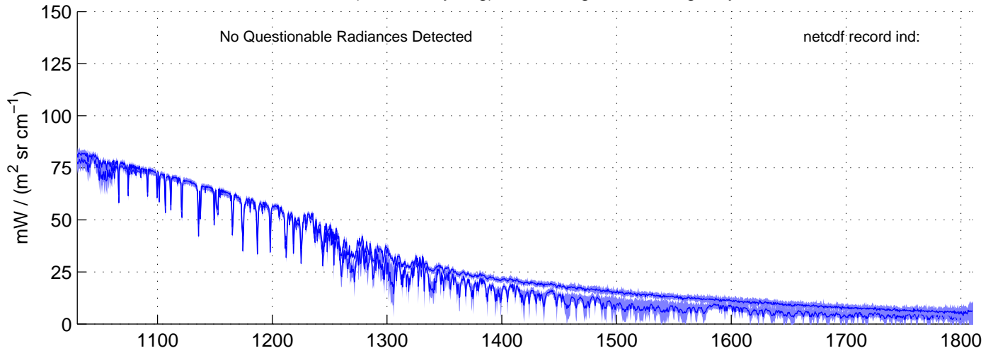
sh130830, REAL(MW) Radiances included in shis_130830_sci_mw.nc BLUE = OK (meaned by seg); RED = significant imaginary content
