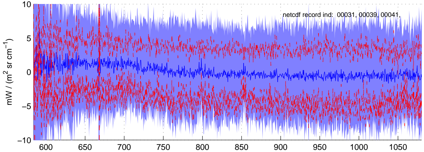
sh130830, Questionable (IMAG) LW Radiances included in shis_130830_sci_lw.nc BLUE = OK (meaned by seg); RED = significant imaginary content
