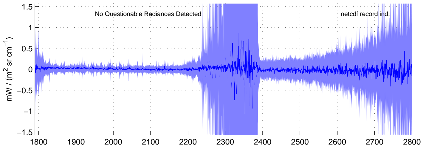
sh130830, PHASE(SW) Radiances included in shis_130830_sci_sw.nc BLUE = OK (meaned by seg); RED = significant imaginary content
