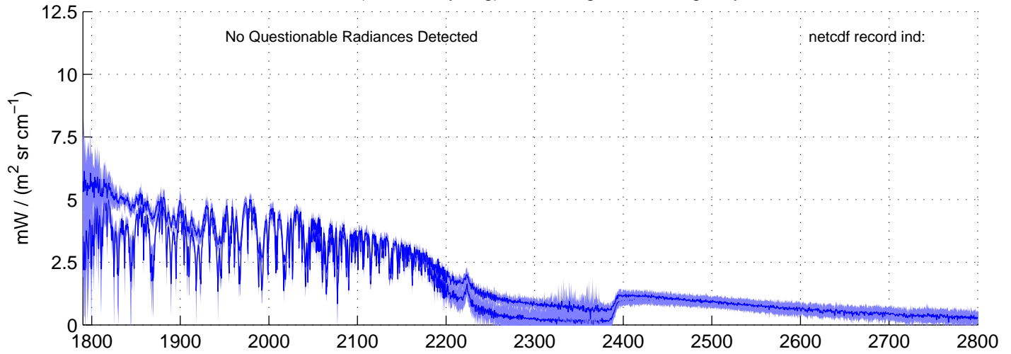
sh130830, REAL(SW) Radiances included in shis_130830_sci_sw.nc BLUE = OK (meaned by seg); RED = significant imaginary content
