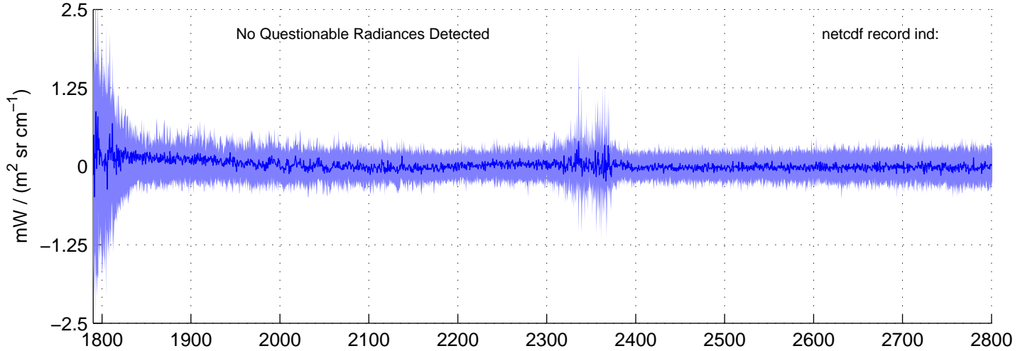
sh130830, IMAG(SW) Radiances included in shis_130830_sci_sw.nc BLUE = OK (meaned by seg); RED = significant imaginary content
