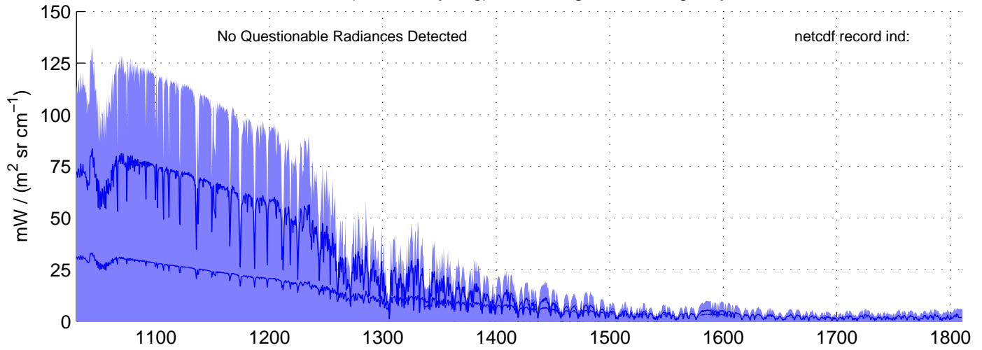
sh130829, REAL(MW) Radiances included in shis_130829_sci_mw.nc BLUE = OK (meaned by seg); RED = significant imaginary content
