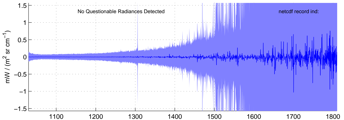
sh130829, PHASE(MW) Radiances included in shis_130829_sci_mw.nc BLUE = OK (meaned by seg); RED = significant imaginary content
