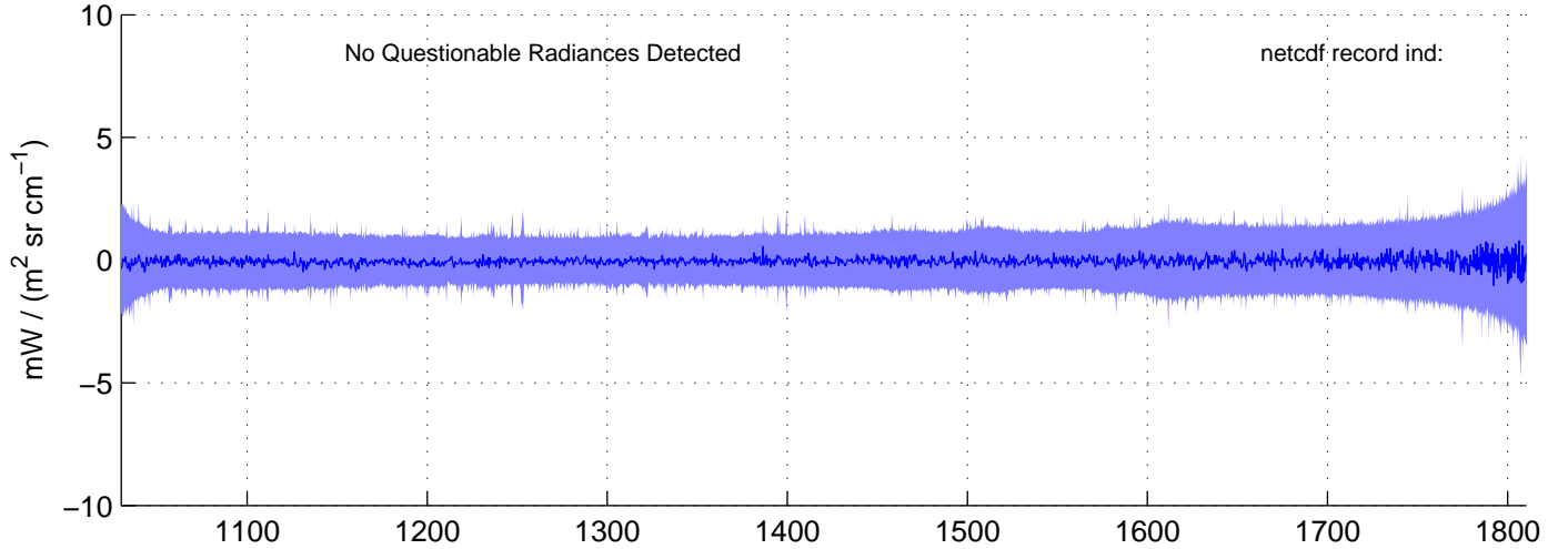
sh130829, IMAG(MW) Radiances included in shis_130829_sci_mw.nc BLUE = OK (meaned by seg); RED = significant imaginary content
