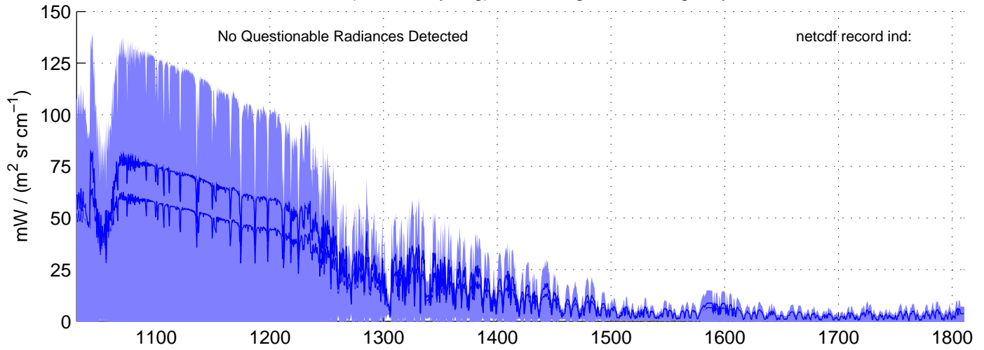
sh130825, REAL(MW) Radiances included in shis_130825_sci_mw.nc BLUE = OK (meaned by seg); RED = significant imaginary content
