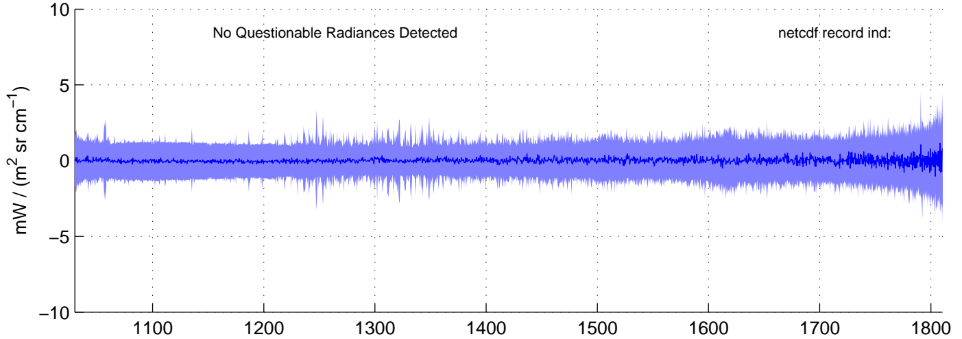
sh130825, IMAG(MW) Radiances included in shis_130825_sci_mw.nc BLUE = OK (meaned by seg); RED = significant imaginary content
