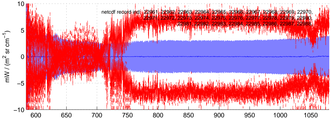
sh130824, Questionable (IMAG) LW Radiances included in shis_130824_sci_lw.nc BLUE = OK (meaned by seg); RED = significant imaginary content
