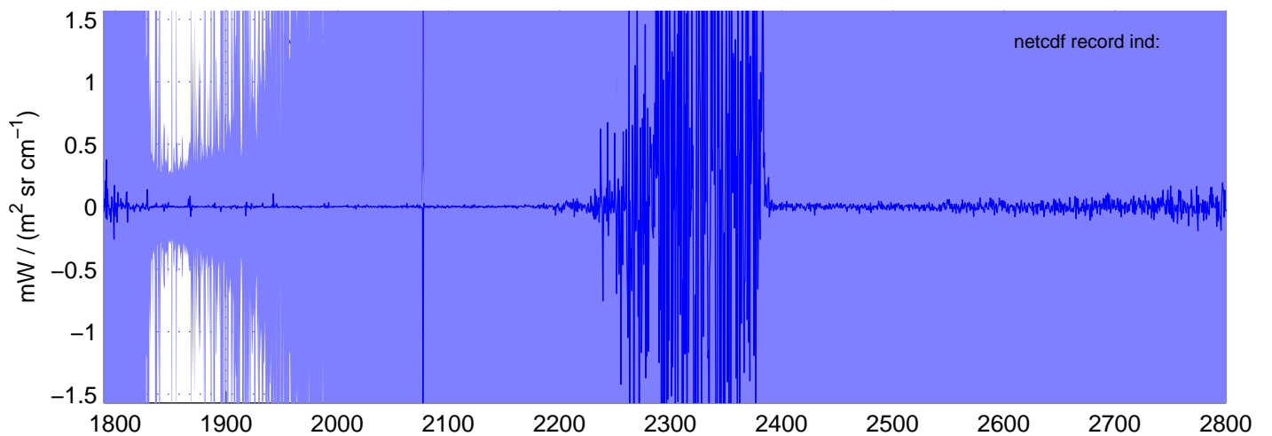
sh130825, PHASE(SW) Radiances included in shis_130825_sci_sw.nc BLUE = OK (meaned by seg); RED = significant imaginary content
