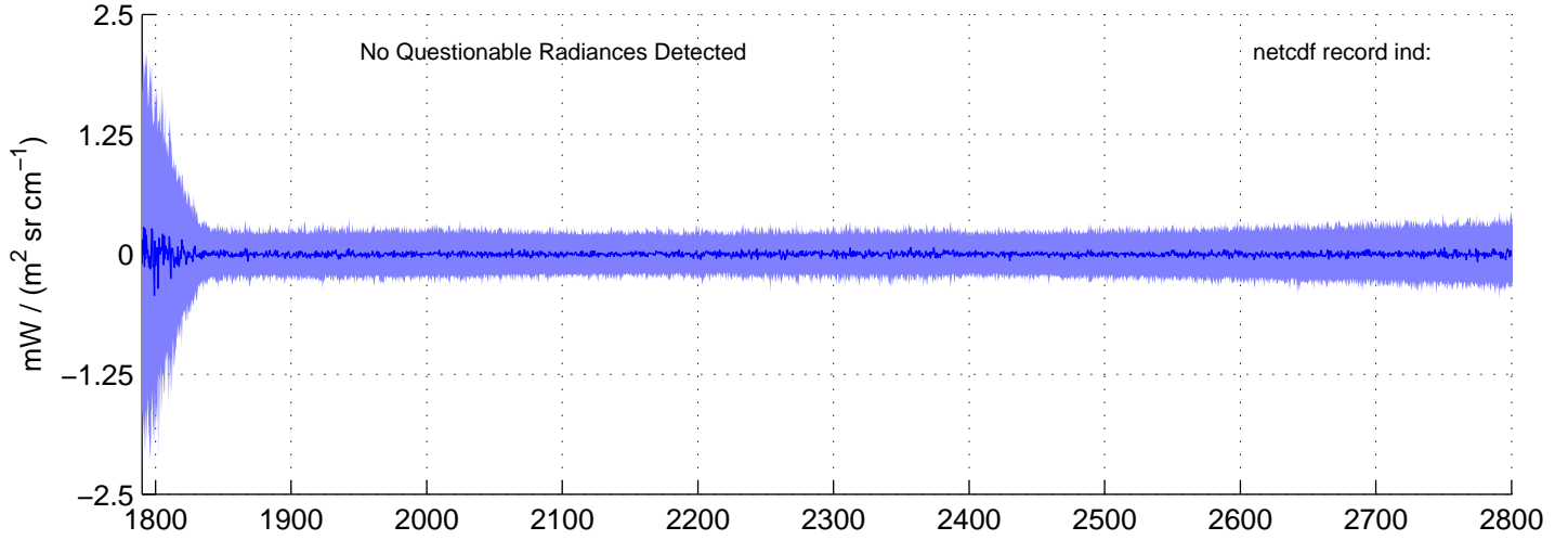
sh130825, IMAG(SW) Radiances included in shis_130825_sci_sw.nc BLUE = OK (meaned by seg); RED = significant imaginary content
