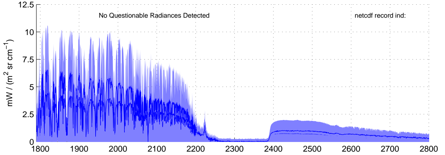
sh130825, REAL(SW) Radiances included in shis_130825_sci_sw.nc BLUE = OK (meaned by seg); RED = significant imaginary content
