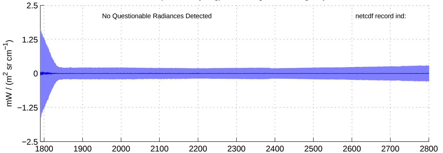
sh130820, IMAG(SW) Radiances included in shis_130820_sci_sw.nc BLUE = OK (meaned by seg); RED = significant imaginary content
