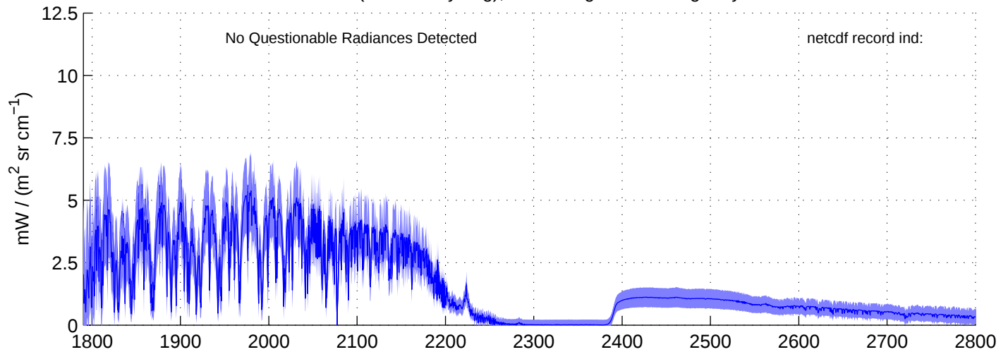
sh130820, REAL(SW) Radiances included in shis_130820_sci_sw.nc BLUE = OK (meaned by seg); RED = significant imaginary content
