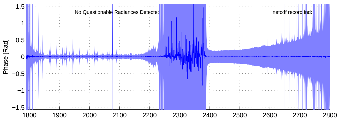
sh130820, PHASE(SW) Radiances included in shis_130820_sci_sw.nc BLUE = OK (meaned by seg); RED = significant imaginary content
