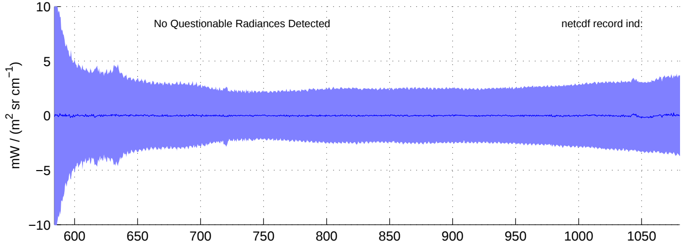
sh130820, Questionable (IMAG) LW Radiances included in shis_130820_sci_lw.nc BLUE = OK (meaned by seg); RED = significant imaginary content
