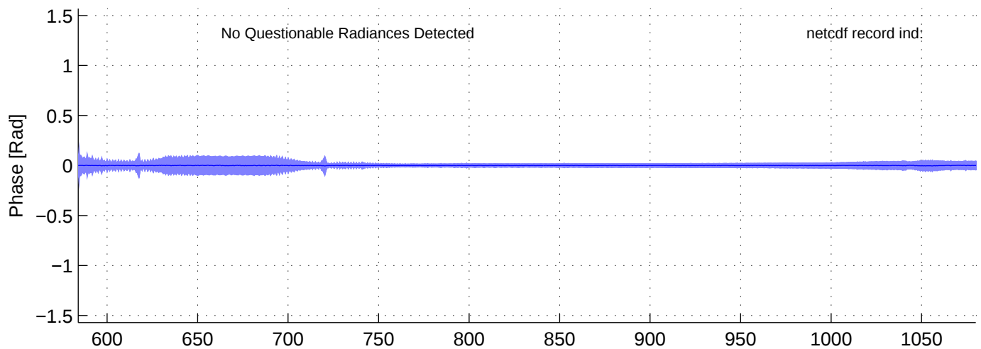
sh130820, PHASE(LW) Radiances included in shis_130820_sci_lw.nc BLUE = OK (meaned by seg); RED = significant imaginary content
