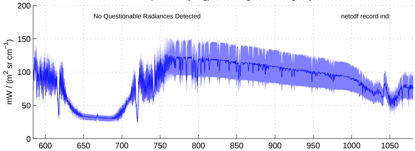
sh130820, REAL(LW) Radiances included in shis_130820_sci_lw.nc BLUE = OK (meaned by seg); RED = significant imaginary content
