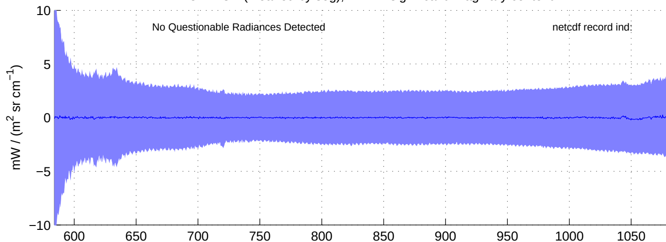
sh130820, Questionable (IMAG) LW Radiances included in shis_130820_sci_lw.nc BLUE = OK (meaned by seg); RED = significant imaginary content
