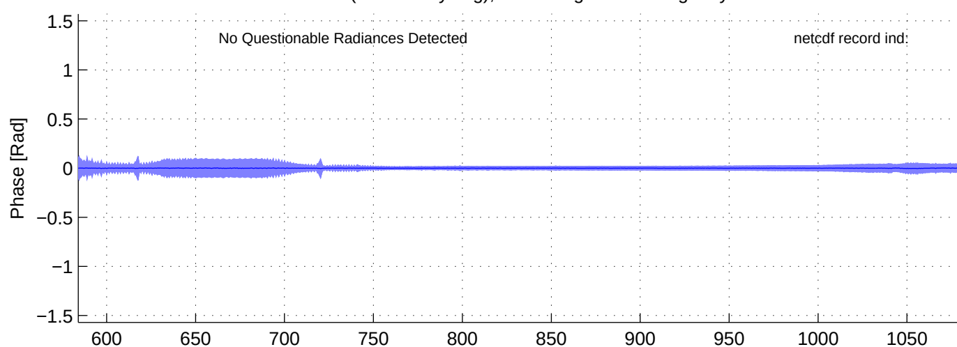
sh130820, PHASE(LW) Radiances included in shis_130820_sci_lw.nc BLUE = OK (meaned by seg); RED = significant imaginary content
