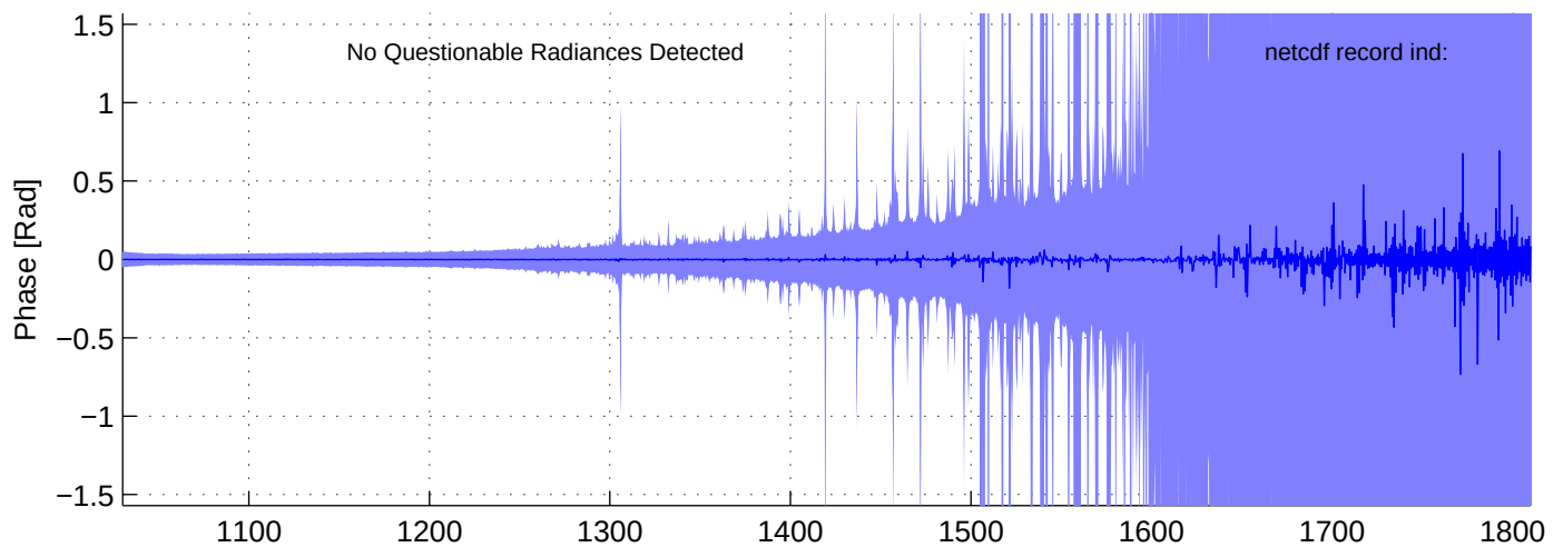
sh130820, PHASE(MW) Radiances included in shis_130820_sci_mw.nc BLUE = OK (meaned by seg); RED = significant imaginary content
