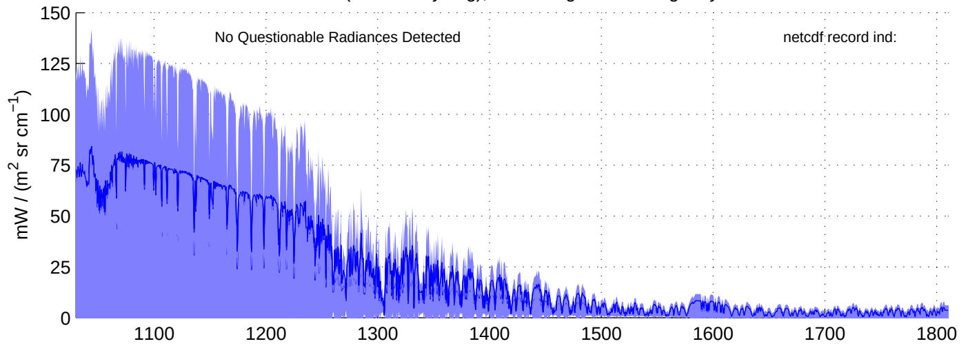
sh130820, REAL(MW) Radiances included in shis_130820_sci_mw.nc BLUE = OK (meaned by seg); RED = significant imaginary content
