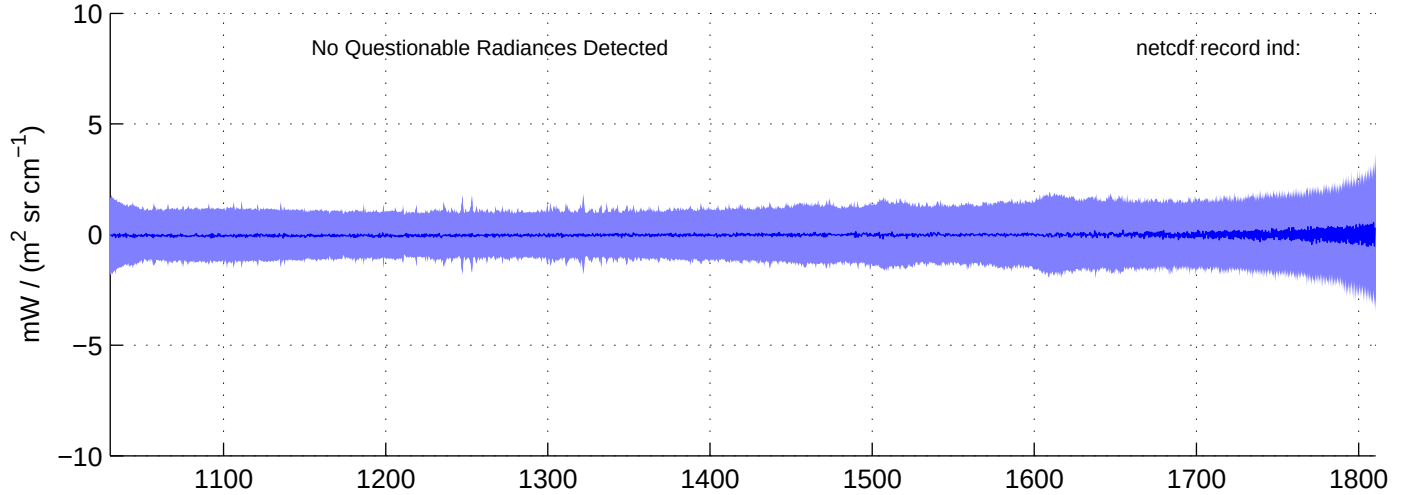
sh130820, IMAG(MW) Radiances included in shis_130820_sci_mw.nc BLUE = OK (meaned by seg); RED = significant imaginary content
