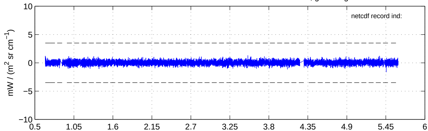
sh130821 Mean IMAG Calibrated Radiance 895.00 – 900.00, good segments
