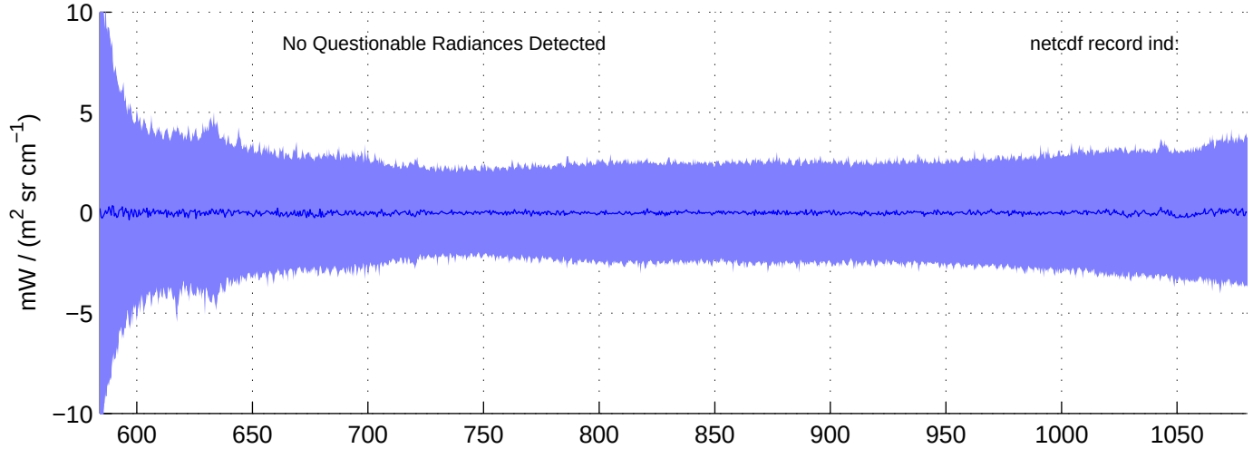
sh130821, Questionable (IMAG) LW Radiances included in shis_130821_sci_lw.nc BLUE = OK (meaned by seg); RED = significant imaginary content
