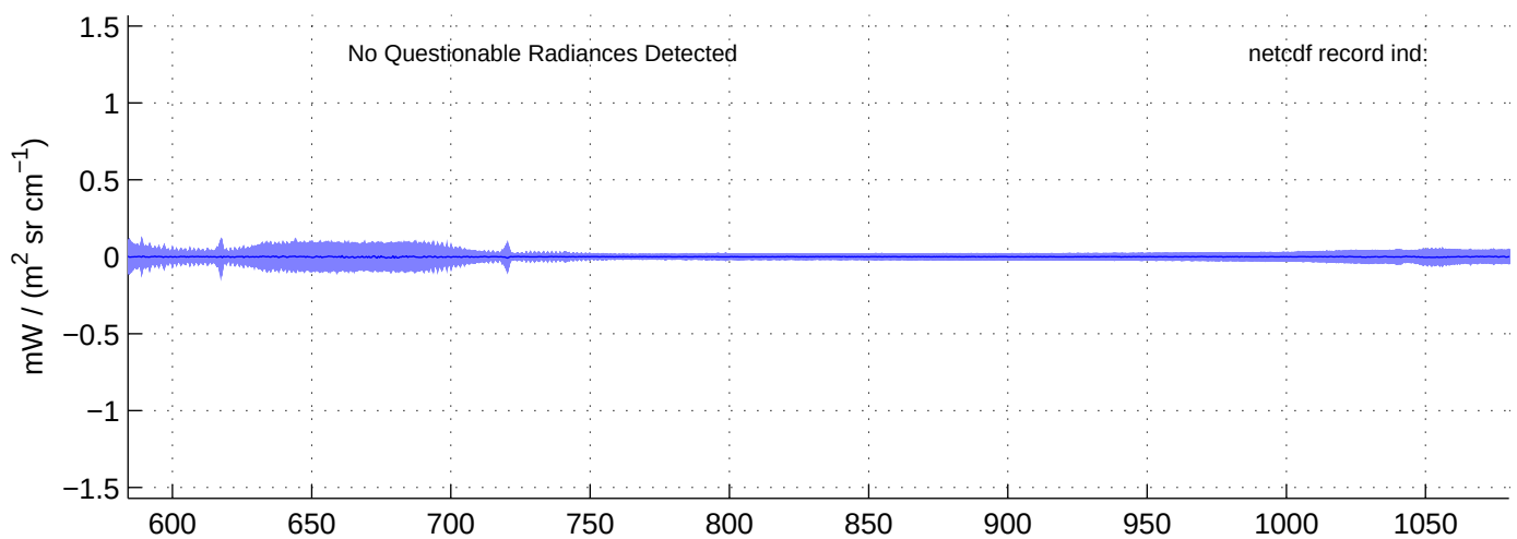
sh130821, PHASE(LW) Radiances included in shis_130821_sci_lw.nc BLUE = OK (meaned by seg); RED = significant imaginary content
