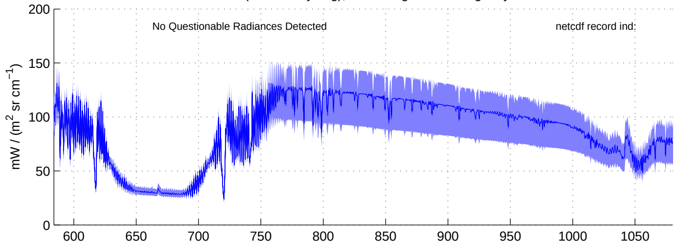
sh130821, REAL(LW) Radiances included in shis_130821_sci_lw.nc BLUE = OK (meaned by seg); RED = significant imaginary content
