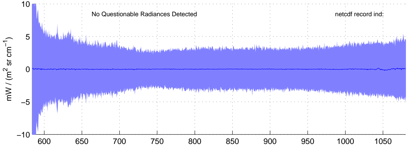
sh130816, Questionable (IMAG) LW Radiances included in shis_130816_sci_lw.nc BLUE = OK (meaned by seg); RED = significant imaginary content
