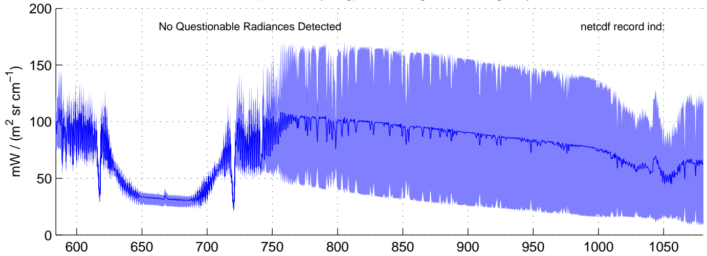
sh130816, REAL(LW) Radiances included in shis_130816_sci_lw.nc BLUE = OK (meaned by seg); RED = significant imaginary content
