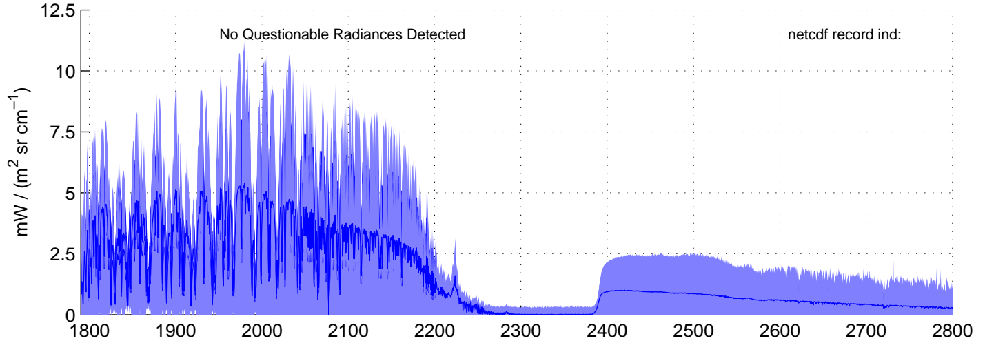
sh130816, REAL(SW) Radiances included in shis_130816_sci_sw.nc BLUE = OK (meaned by seg); RED = significant imaginary content
