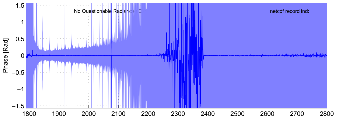
sh130816, PHASE(SW) Radiances included in shis_130816_sci_sw.nc BLUE = OK (meaned by seg); RED = significant imaginary content
