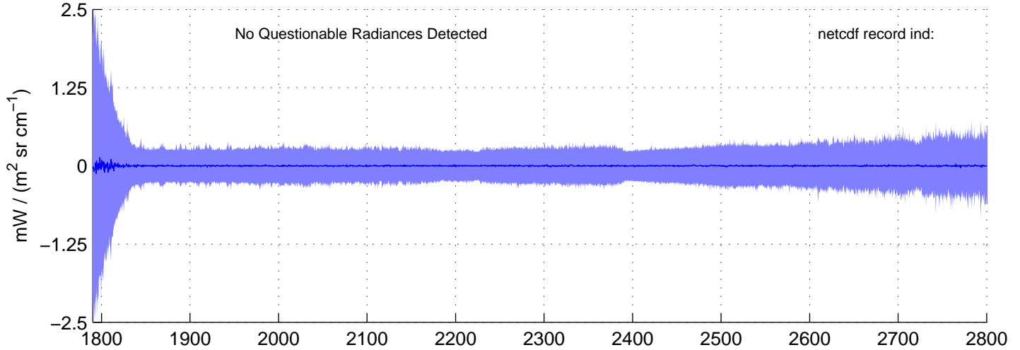
sh130816, IMAG(SW) Radiances included in shis_130816_sci_sw.nc BLUE = OK (meaned by seg); RED = significant imaginary content
