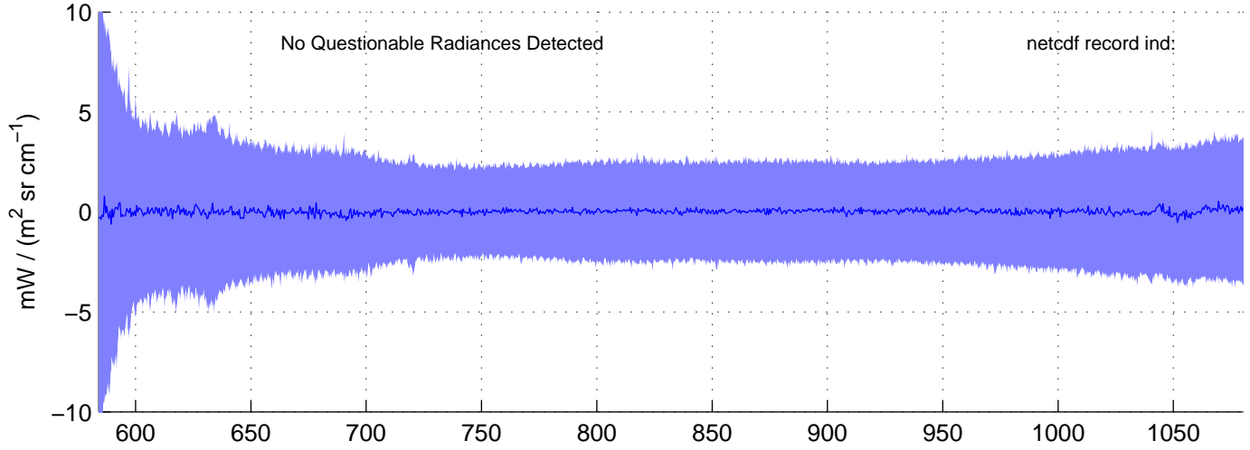
sh130816, Questionable (IMAG) LW Radiances included in shis_130816_sci_lw.nc BLUE = OK (meaned by seg); RED = significant imaginary content
