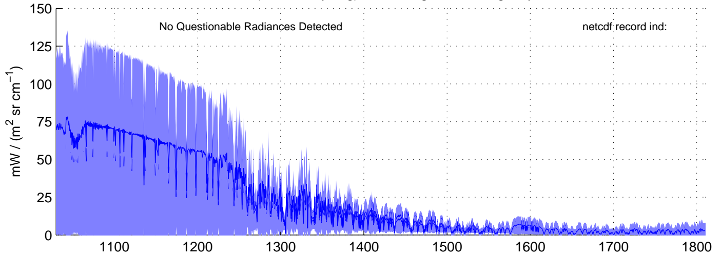
sh130816, REAL(MW) Radiances included in shis_130816_sci_mw.nc BLUE = OK (meaned by seg); RED = significant imaginary content
