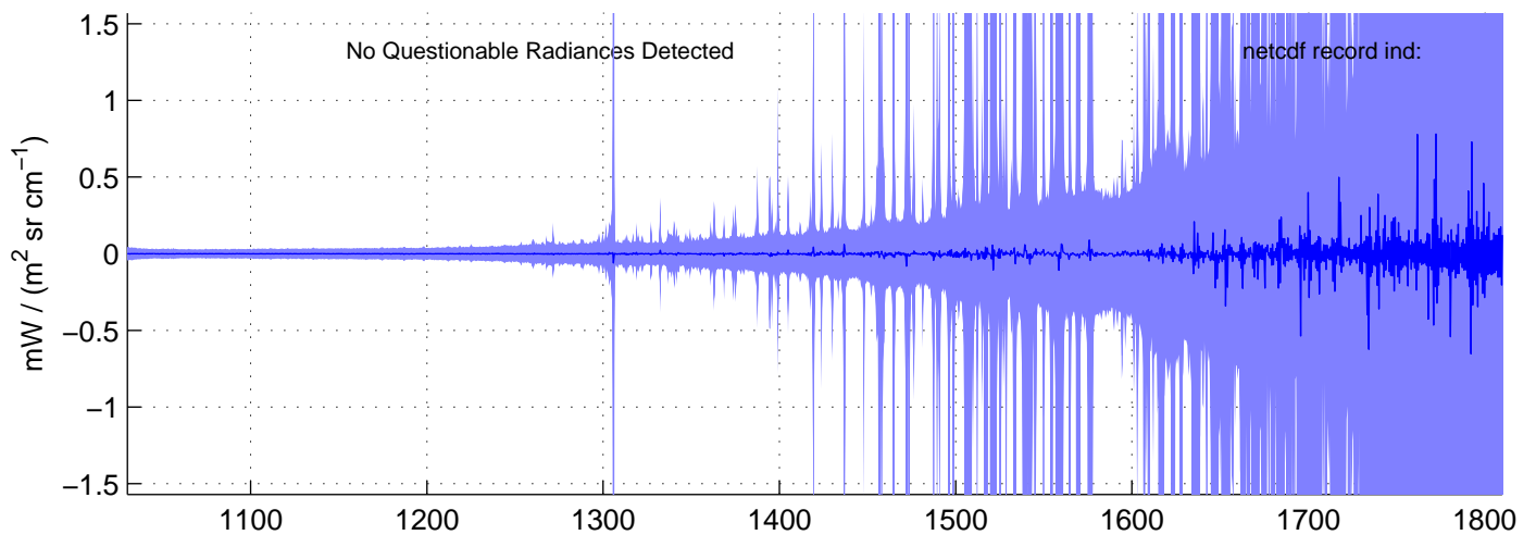
sh130816, PHASE(MW) Radiances included in shis_130816_sci_mw.nc BLUE = OK (meaned by seg); RED = significant imaginary content
