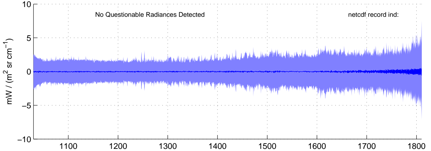
sh130816, IMAG(MW) Radiances included in shis_130816_sci_mw.nc BLUE = OK (meaned by seg); RED = significant imaginary content
