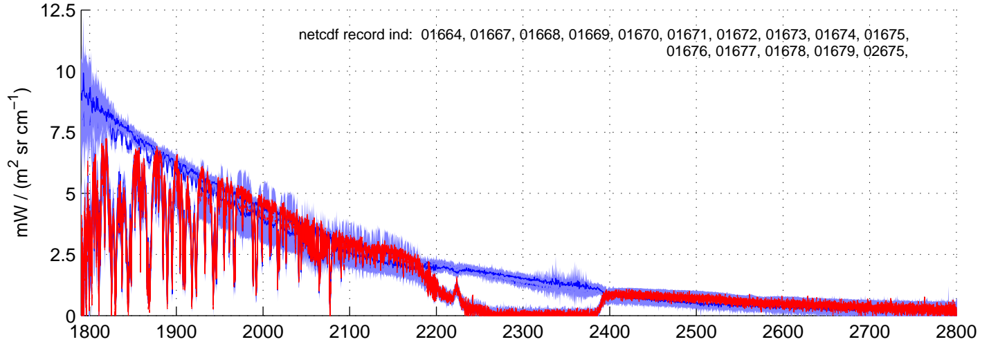
sh130530, REAL(SW) Radiances included in shis_130530_sci_sw.nc BLUE = OK (meaned by seg); RED = significant imaginary content
