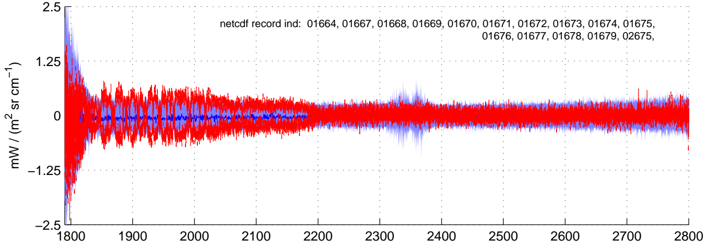
sh130530, IMAG(SW) Radiances included in shis_130530_sci_sw.nc BLUE = OK (meaned by seg); RED = significant imaginary content
