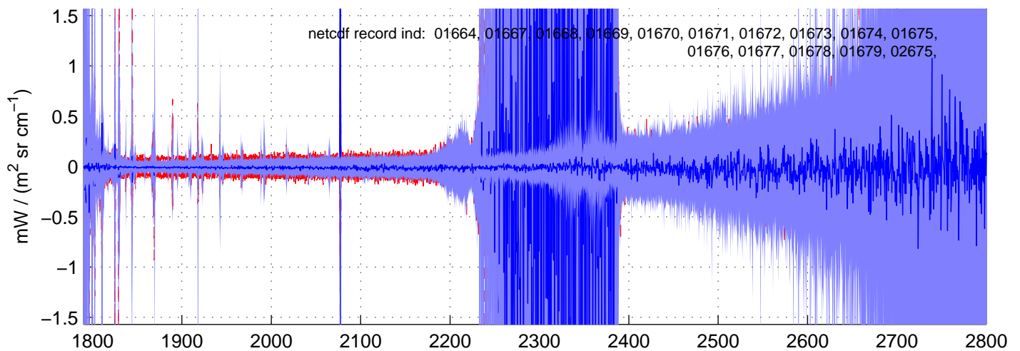
sh130530, PHASE(SW) Radiances included in shis_130530_sci_sw.nc BLUE = OK (meaned by seg); RED = significant imaginary content
