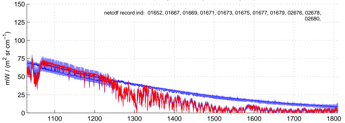
sh130530, REAL(MW) Radiances included in shis_130530_sci_mw.nc BLUE = OK (meaned by seg); RED = significant imaginary content
