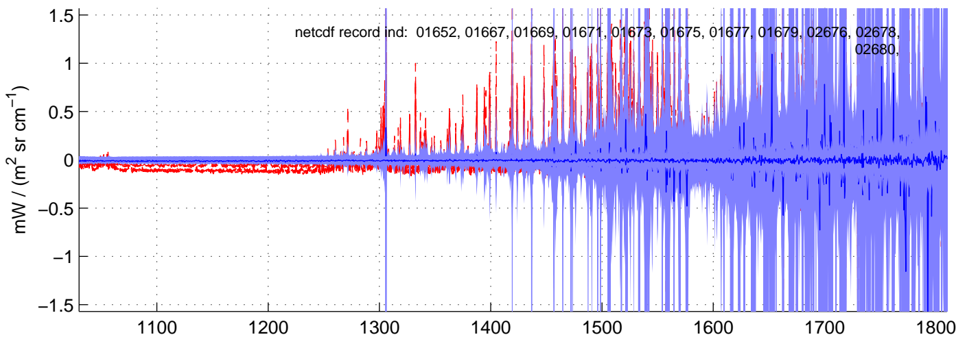
sh130530, PHASE(MW) Radiances included in shis_130530_sci_mw.nc BLUE = OK (meaned by seg); RED = significant imaginary content
