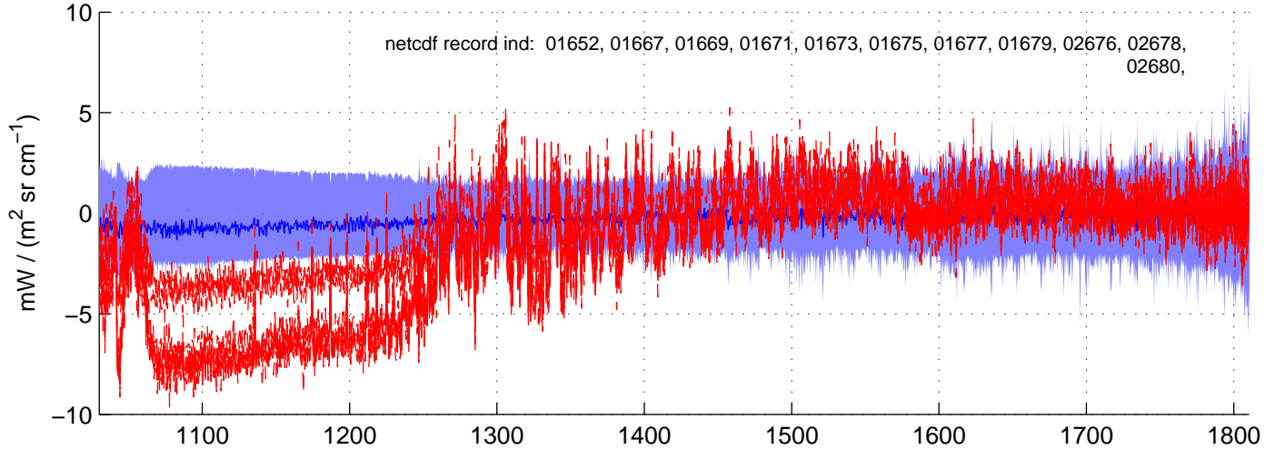
sh130530, IMAG(MW) Radiances included in shis_130530_sci_mw.nc BLUE = OK (meaned by seg); RED = significant imaginary content
