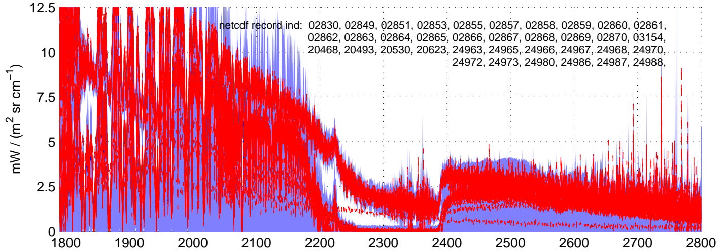
sh130524, REAL(SW) Radiances included in shis_130524_sci_sw.nc BLUE = OK (meaned by seg); RED = significant imaginary content
