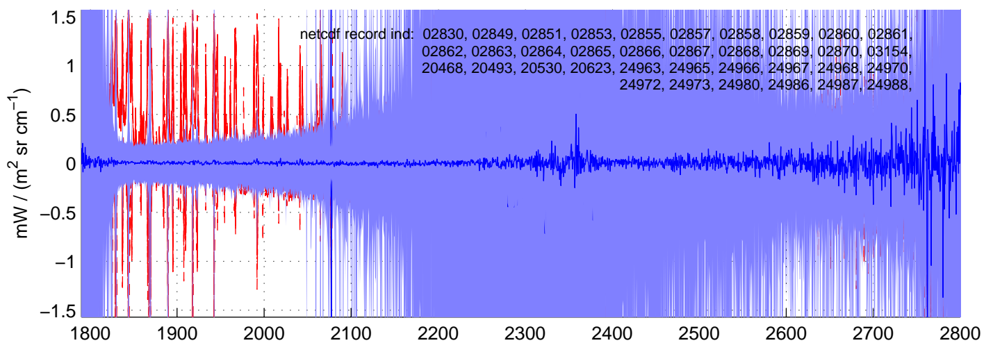
sh130524, PHASE(SW) Radiances included in shis_130524_sci_sw.nc BLUE = OK (meaned by seg); RED = significant imaginary content
