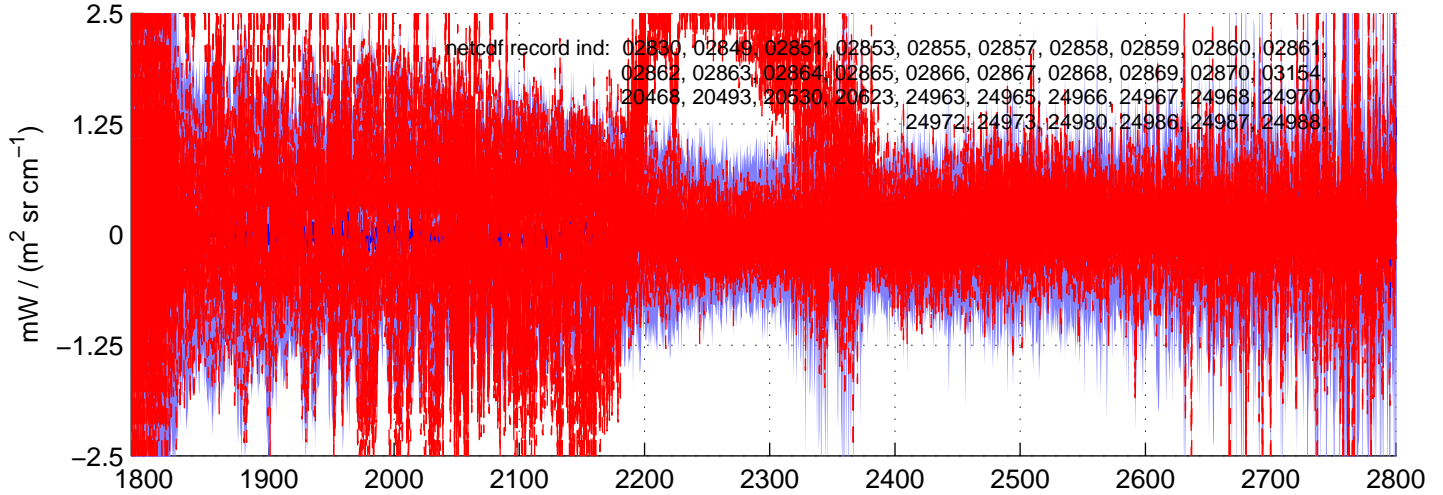
sh130524, IMAG(SW) Radiances included in shis_130524_sci_sw.nc BLUE = OK (meaned by seg); RED = significant imaginary content
