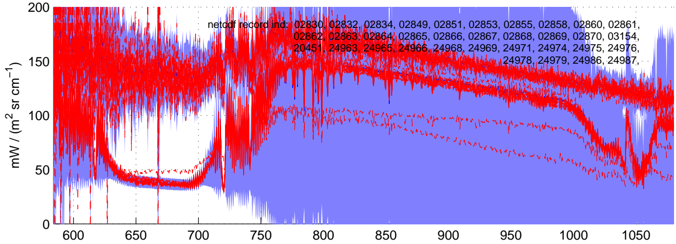
sh130524, REAL(LW) Radiances included in shis_130524_sci_lw.nc BLUE = OK (meaned by seg); RED = significant imaginary content
