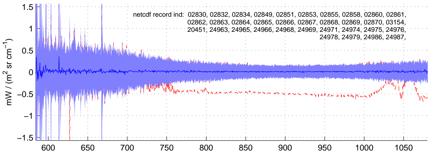
sh130524, PHASE(LW) Radiances included in shis_130524_sci_lw.nc BLUE = OK (meaned by seg); RED = significant imaginary content
