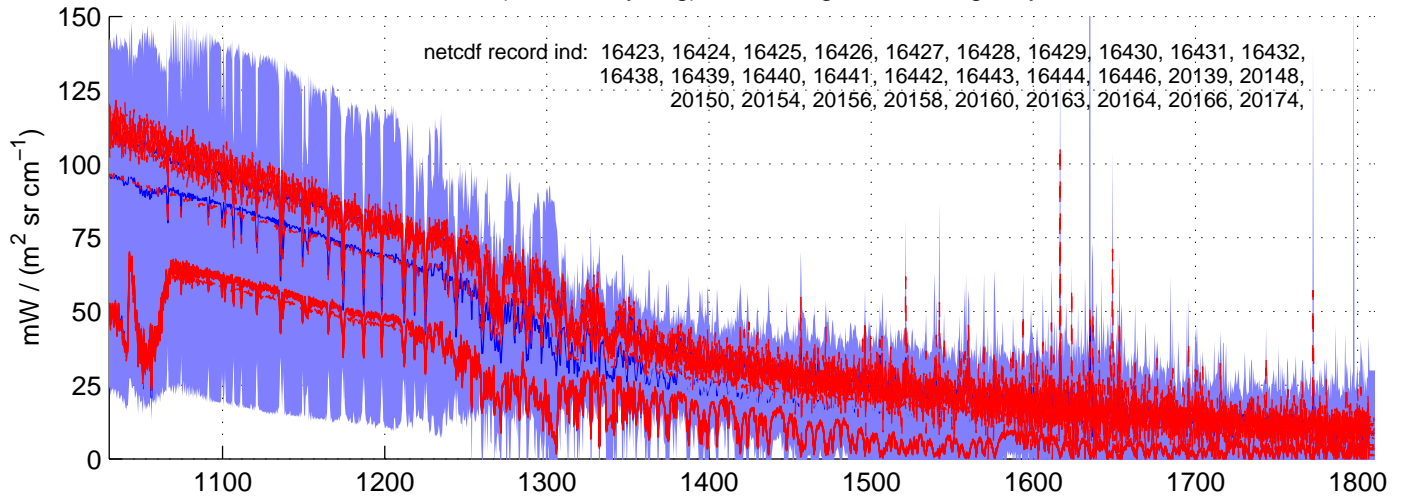
sh130523, REAL(MW) Radiances included in shis_130523_sci_mw.nc BLUE = OK (meaned by seg); RED = significant imaginary content
