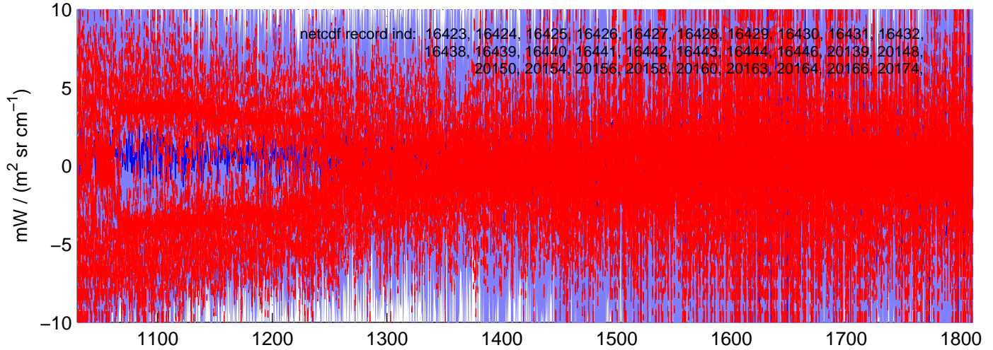
sh130523, IMAG(MW) Radiances included in shis_130523_sci_mw.nc BLUE = OK (meaned by seg); RED = significant imaginary content
