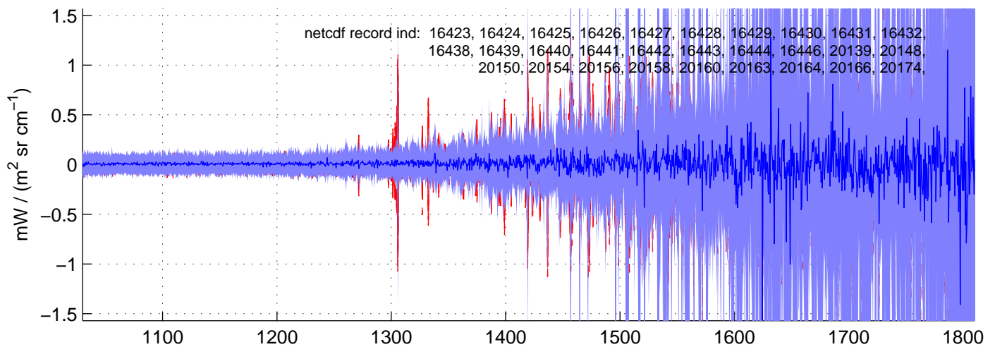
sh130523, PHASE(MW) Radiances included in shis_130523_sci_mw.nc BLUE = OK (meaned by seg); RED = significant imaginary content
