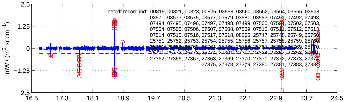
sh130522 Mean IMAG Calibrated Radiance 2000.00 – 2025.00, good segments
