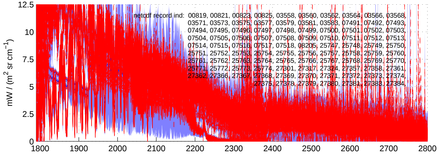
sh130522, REAL(SW) Radiances included in shis_130522_sci_sw.nc BLUE = OK (meaned by seg); RED = significant imaginary content
