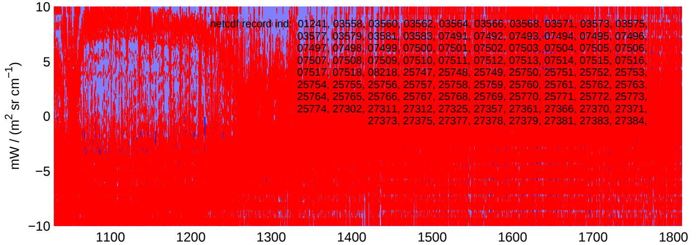
sh130522, IMAG(MW) Radiances included in shis_130522_sci_mw.nc BLUE = OK (meaned by seg); RED = significant imaginary content
