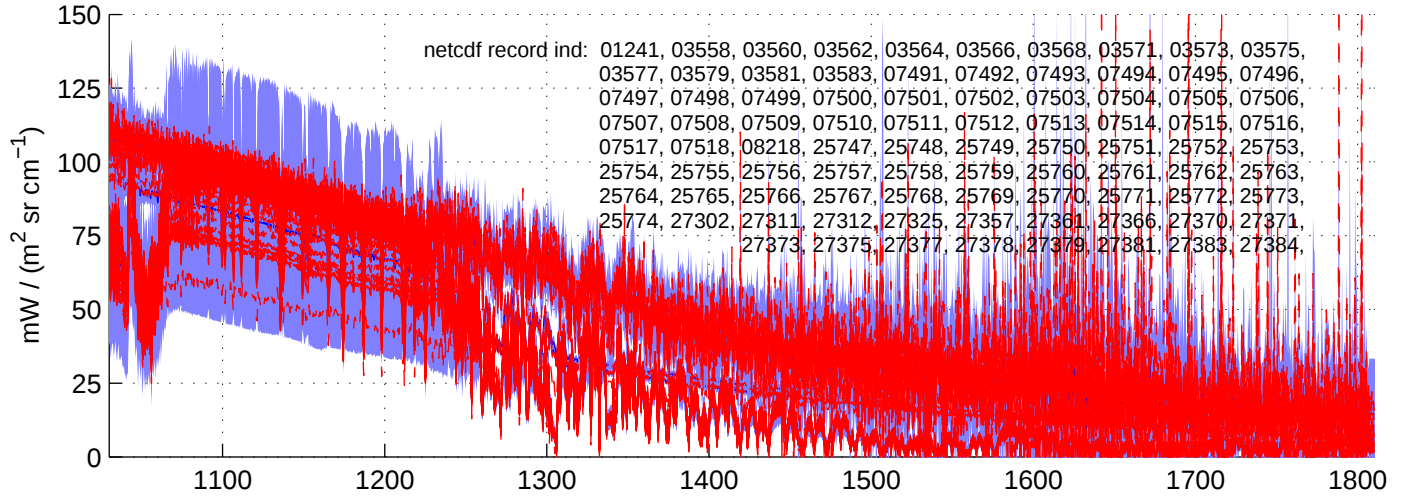
sh130522, REAL(MW) Radiances included in shis_130522_sci_mw.nc BLUE = OK (meaned by seg); RED = significant imaginary content
