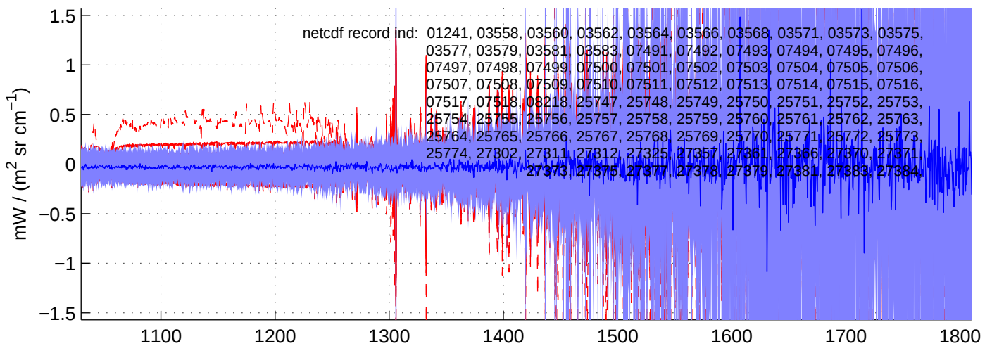
sh130522, PHASE(MW) Radiances included in shis_130522_sci_mw.nc BLUE = OK (meaned by seg); RED = significant imaginary content
