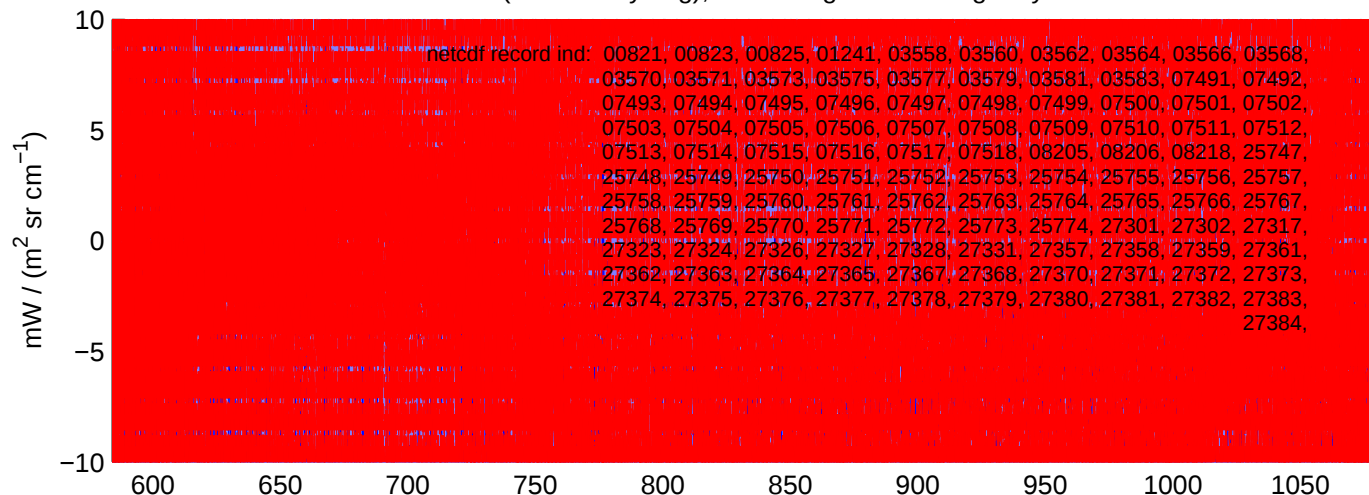
sh130522, Questionable (IMAG) LW Radiances included in shis_130522_sci_lw.nc BLUE = OK (meaned by seg); RED = significant imaginary content
