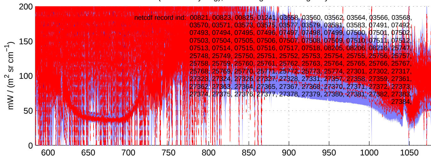
sh130522, REAL(LW) Radiances included in shis_130522_sci_lw.nc BLUE = OK (meaned by seg); RED = significant imaginary content
