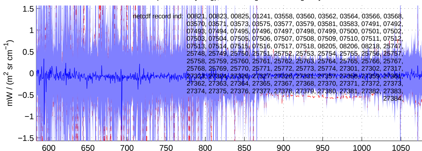
sh130522, PHASE(LW) Radiances included in shis_130522_sci_lw.nc BLUE = OK (meaned by seg); RED = significant imaginary content
