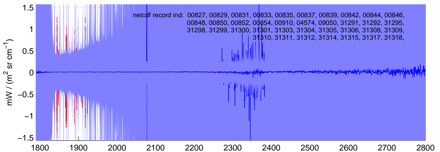
sh130520, PHASE(SW) Radiances included in shis_130520_sci_sw.nc BLUE = OK (meaned by seg); RED = significant imaginary content
