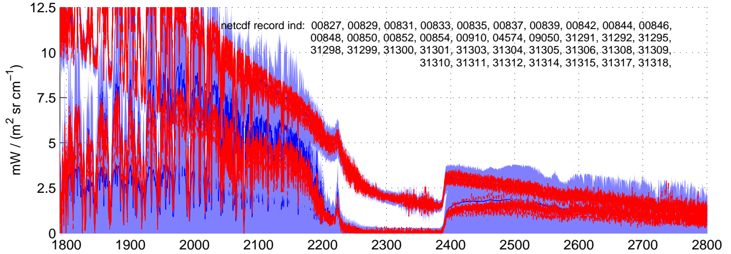
sh130520, REAL(SW) Radiances included in shis_130520_sci_sw.nc BLUE = OK (meaned by seg); RED = significant imaginary content
