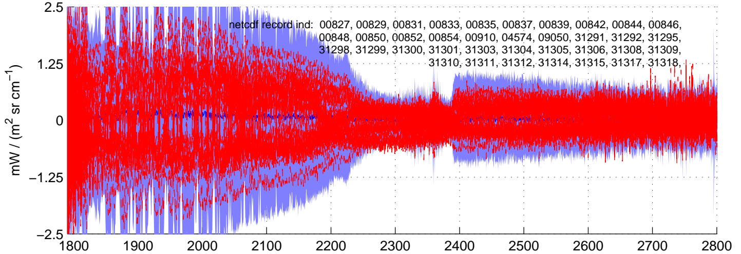
sh130520, IMAG(SW) Radiances included in shis_130520_sci_sw.nc BLUE = OK (meaned by seg); RED = significant imaginary content
