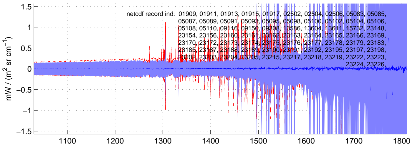
sh130518, PHASE(MW) Radiances included in shis_130518_sci_mw.nc BLUE = OK (meaned by seg); RED = significant imaginary content
