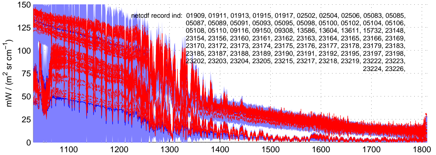
sh130518, REAL(MW) Radiances included in shis_130518_sci_mw.nc BLUE = OK (meaned by seg); RED = significant imaginary content
