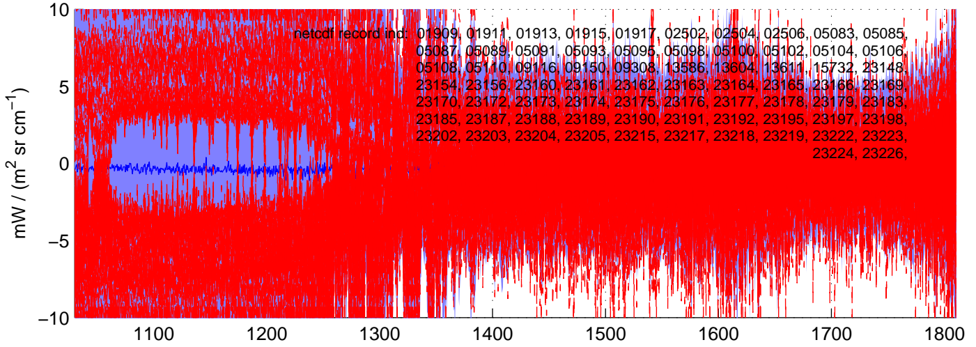
sh130518, IMAG(MW) Radiances included in shis_130518_sci_mw.nc BLUE = OK (meaned by seg); RED = significant imaginary content
