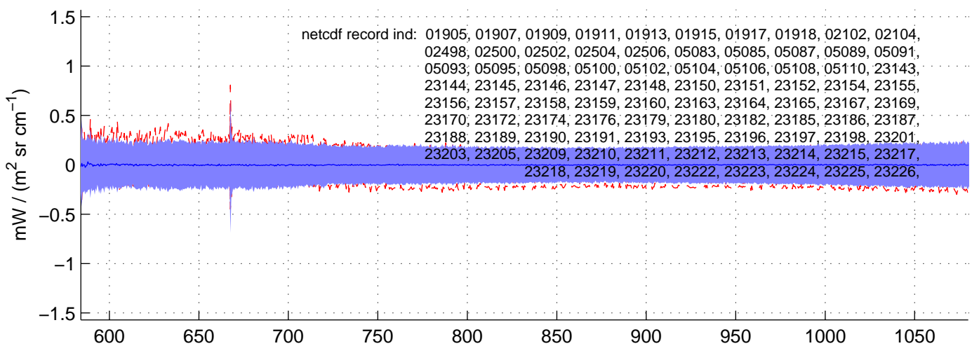
sh130518, PHASE(LW) Radiances included in shis_130518_sci_lw.nc BLUE = OK (meaned by seg); RED = significant imaginary content
