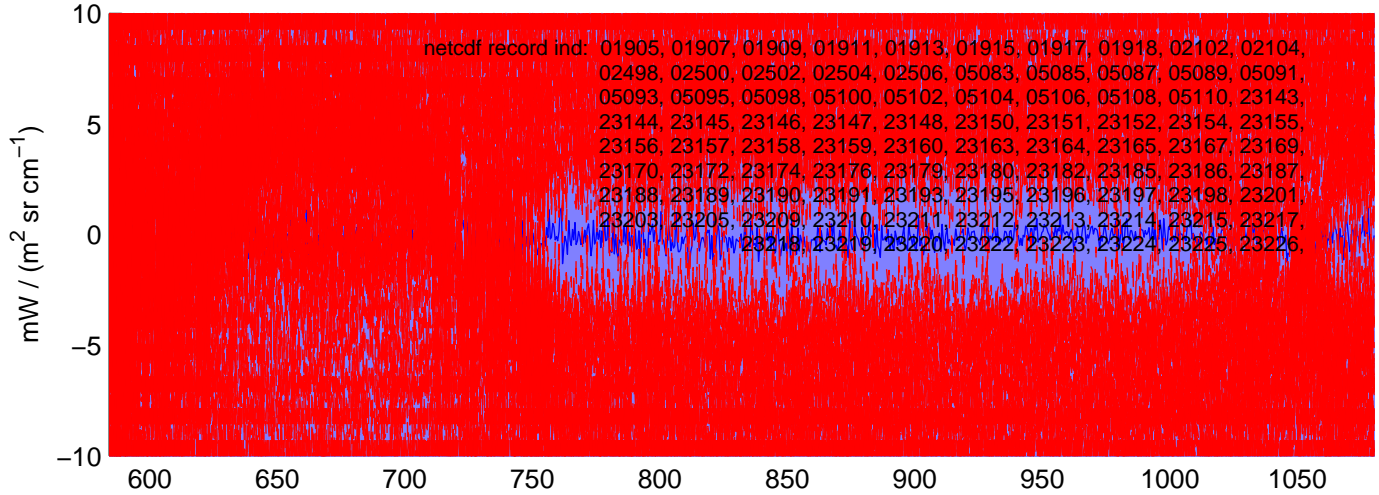
sh130518, Questionable (IMAG) LW Radiances included in shis_130518_sci_lw.nc BLUE = OK (meaned by seg); RED = significant imaginary content
