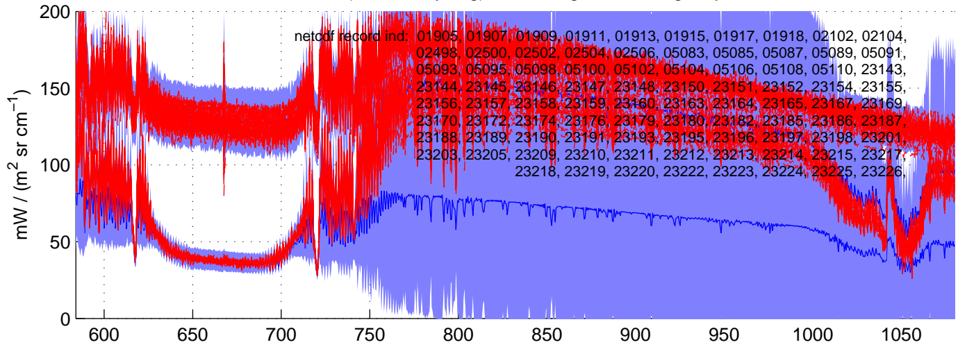
sh130518, REAL(LW) Radiances included in shis_130518_sci_lw.nc BLUE = OK (meaned by seg); RED = significant imaginary content
