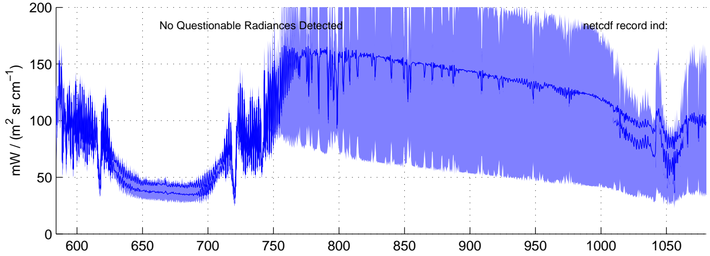
sh130515, REAL(LW) Radiances included in shis_130515_sci_lw.nc BLUE = OK (meaned by seg); RED = significant imaginary content
