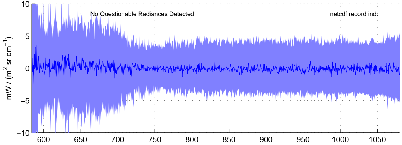
sh130515, Questionable (IMAG) LW Radiances included in shis_130515_sci_lw.nc BLUE = OK (meaned by seg); RED = significant imaginary content
