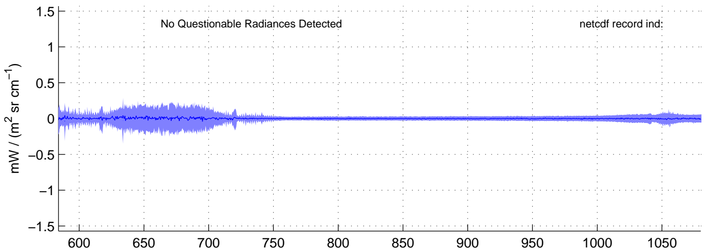
sh130515, PHASE(LW) Radiances included in shis_130515_sci_lw.nc BLUE = OK (meaned by seg); RED = significant imaginary content
