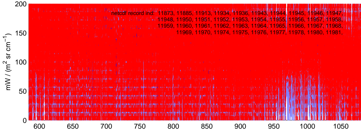
sh130510, REAL(LW) Radiances included in shis_130510_sci_lw.nc BLUE = OK (meaned by seg); RED = significant imaginary content
