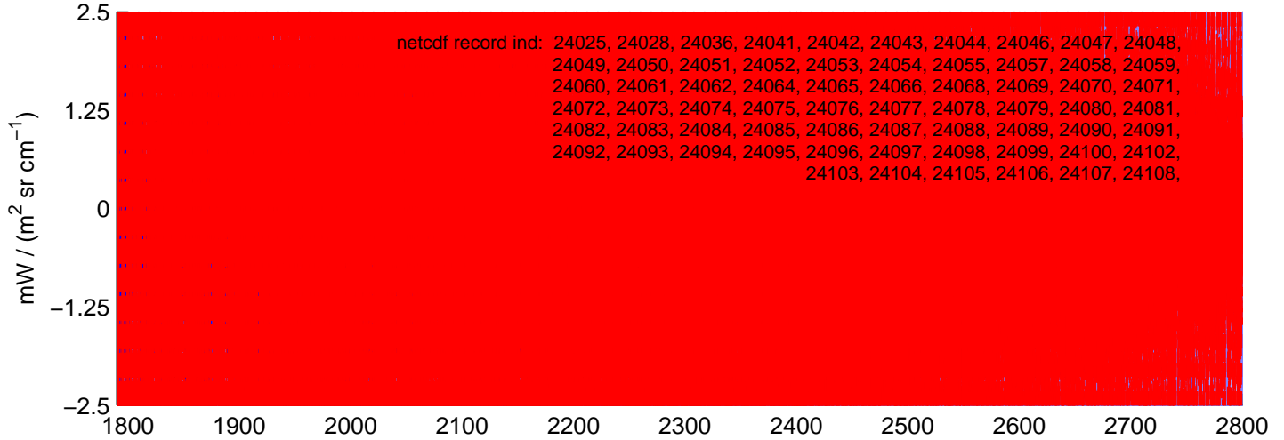
sh130507, IMAG(SW) Radiances included in shis_130507_sci_sw.nc BLUE = OK (meaned by seg); RED = significant imaginary content
