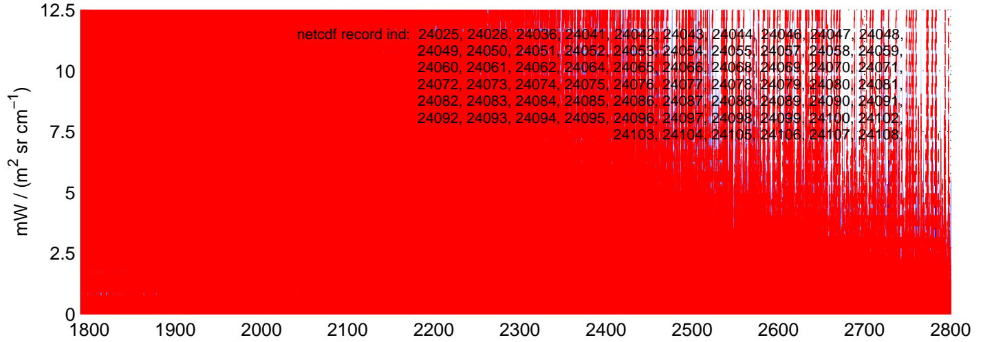
sh130507, REAL(SW) Radiances included in shis_130507_sci_sw.nc BLUE = OK (meaned by seg); RED = significant imaginary content
