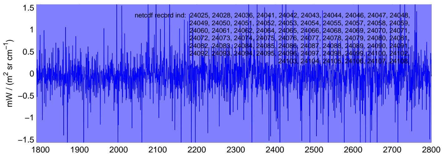
sh130507, PHASE(SW) Radiances included in shis_130507_sci_sw.nc BLUE = OK (meaned by seg); RED = significant imaginary content
