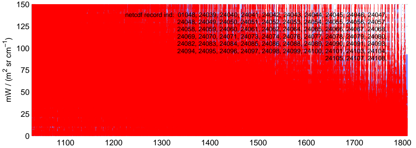
sh130507, REAL(MW) Radiances included in shis_130507_sci_mw.nc BLUE = OK (meaned by seg); RED = significant imaginary content
