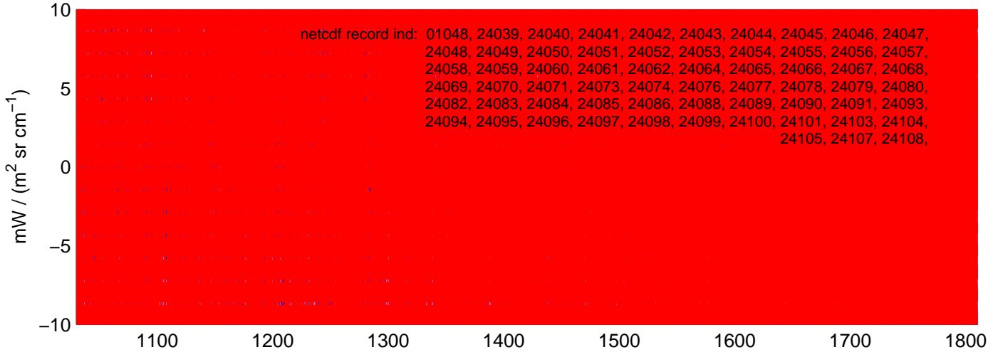
sh130507, IMAG(MW) Radiances included in shis_130507_sci_mw.nc BLUE = OK (meaned by seg); RED = significant imaginary content
