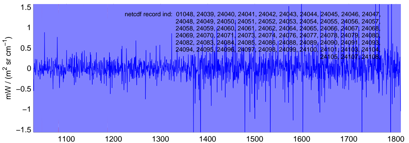
sh130507, PHASE(MW) Radiances included in shis_130507_sci_mw.nc BLUE = OK (meaned by seg); RED = significant imaginary content
